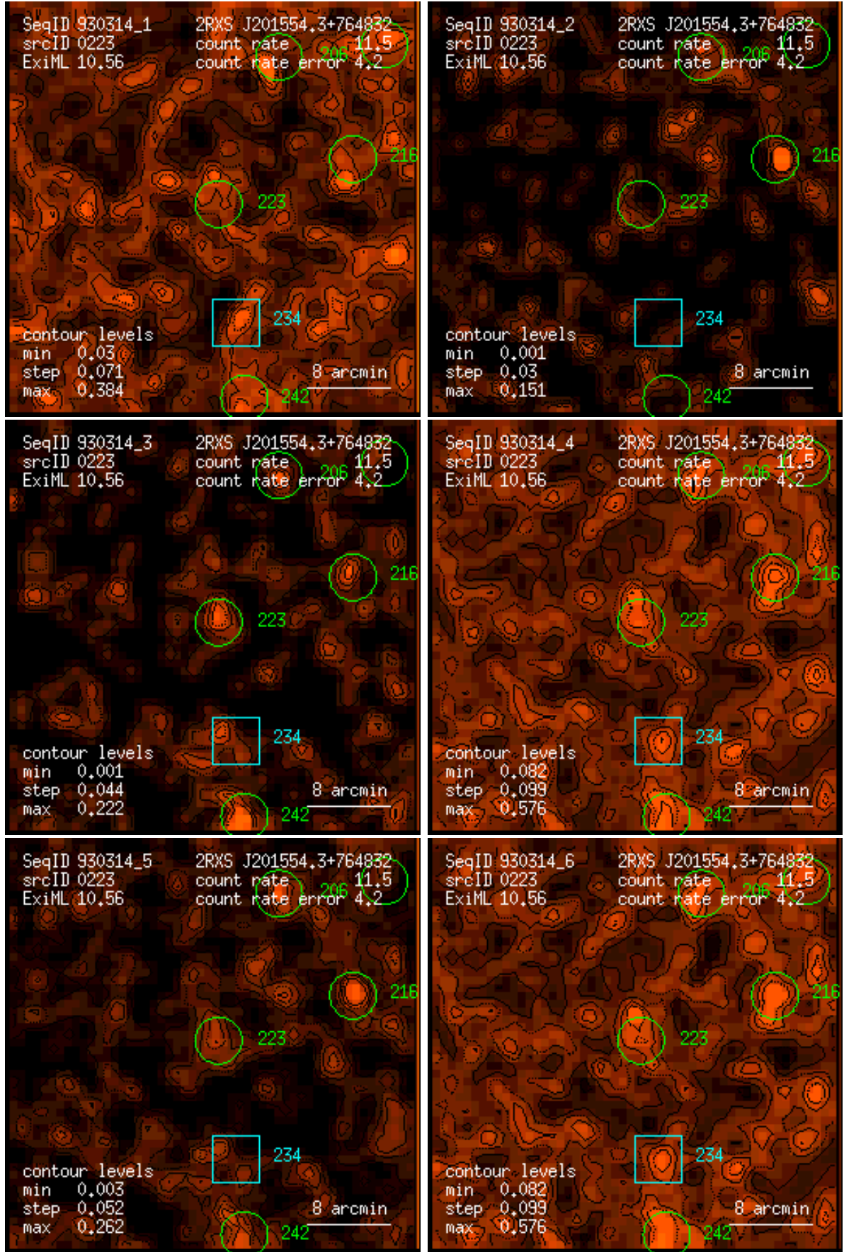
Figure 223: RASS 930314: detection 0223: band rate images, Gaussian filter: (1) PSPC channels 11 – 41, (2) 52 – 90, (3) 91 – 201, (4) 11 – 235, (5) 52 – 201, (6) 11 – 201. Broad band rates in counts/ks. Band rate contour levels in counts/ks/arcmin 2 .
