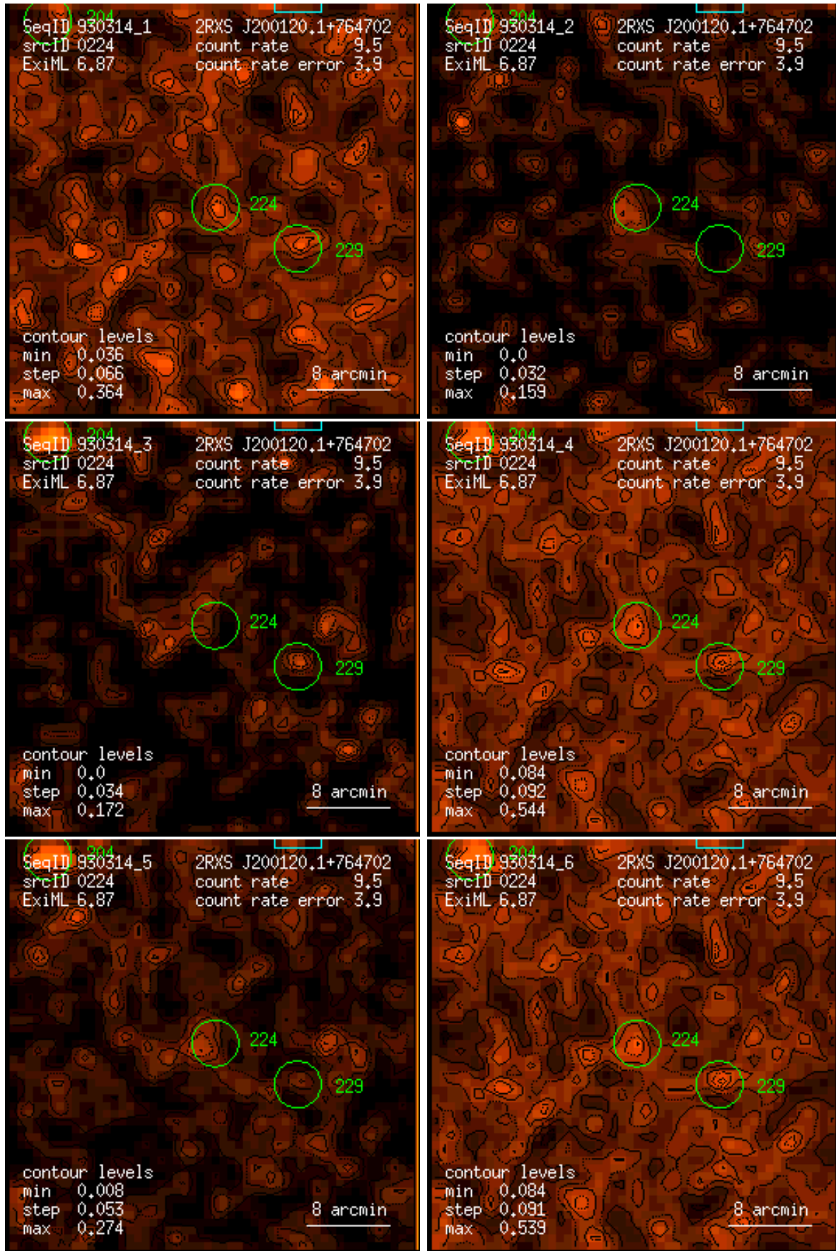
Figure 224: RASS 930314: detection 0224: band rate images, Gaussian filter: (1) PSPC channels 11 – 41, (2) 52 – 90, (3) 91 – 201, (4) 11 – 235, (5) 52 – 201, (6) 11 – 201. Broad band rates in counts/ks. Band rate contour levels in counts/ks/arcmin 2 .
