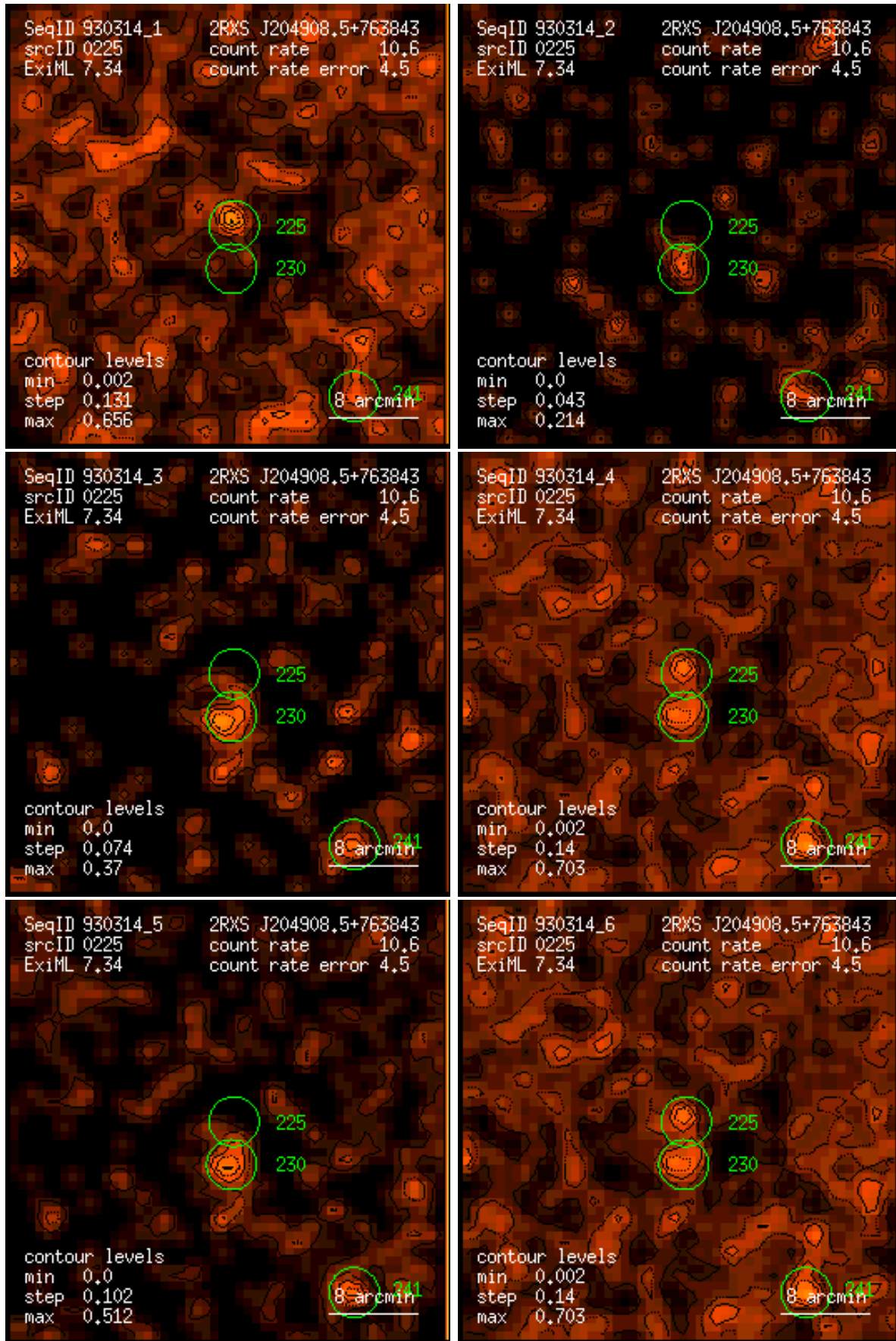
Figure 225: RASS 930314: detection 0225: band rate images, Gaussian filter: (1) PSPC channels 11 – 41, (2) 52 – 90, (3) 91 – 201, (4) 11 – 235, (5) 52 – 201, (6) 11 – 201. Broad band rates in counts/ks. Band rate contour levels in counts/ks/arcmin 2 .
