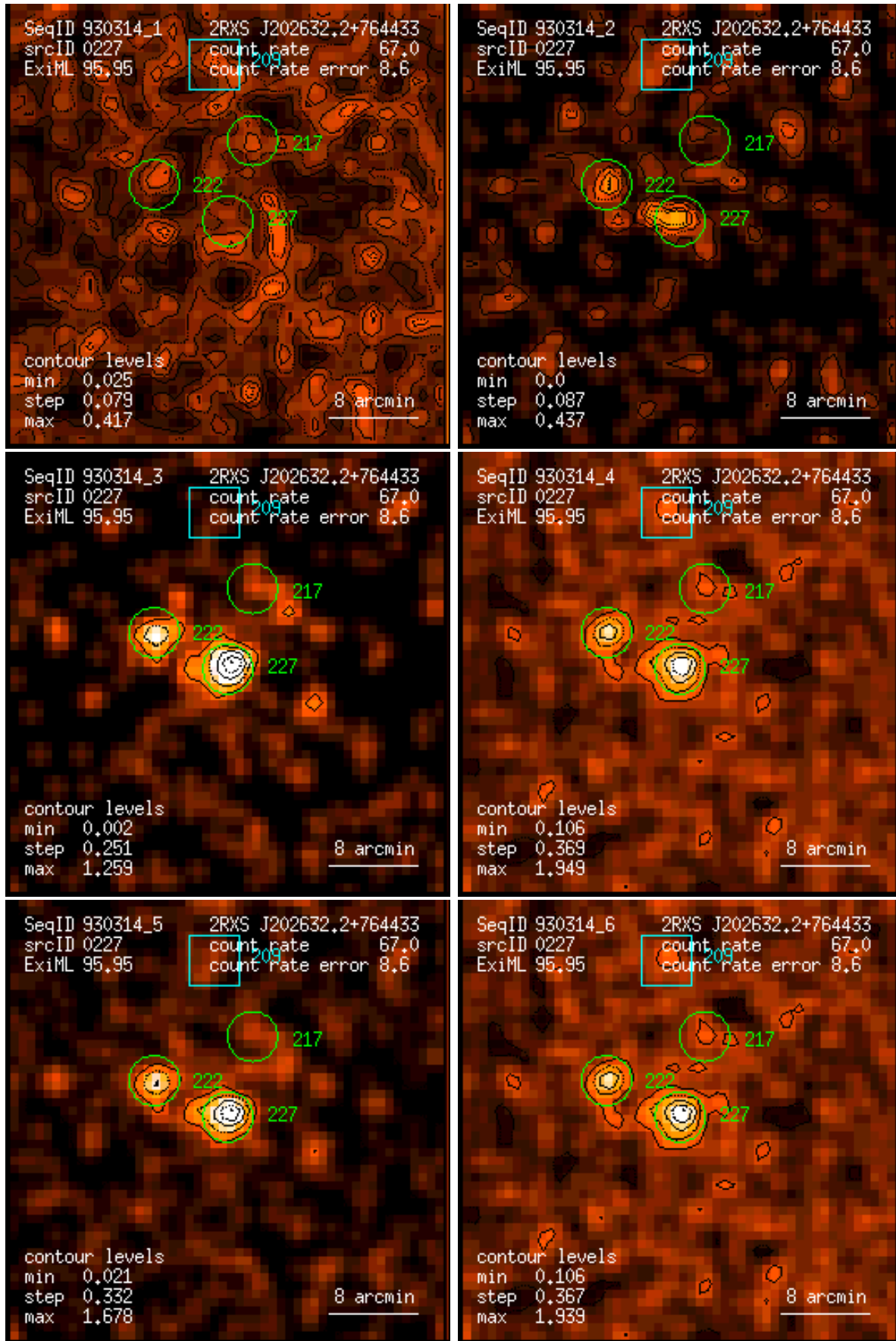
Figure 227: RASS 930314: detection 0227: band rate images, Gaussian filter: (1) PSPC channels 11 – 41, (2) 52 – 90, (3) 91 – 201, (4) 11 – 235, (5) 52 – 201, (6) 11 – 201. Broad band rates in counts/ks. Band rate contour levels in counts/ks/arcmin 2 .
