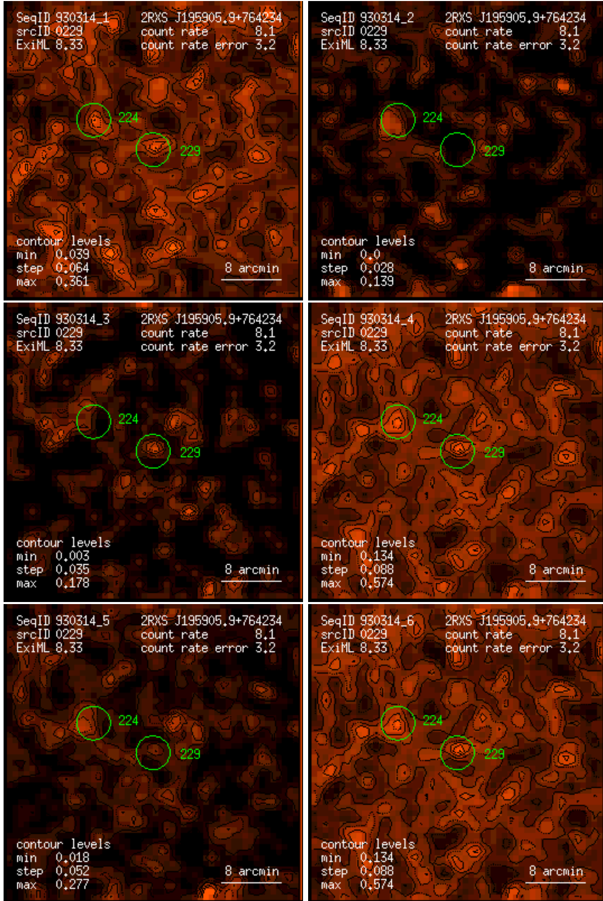
Figure 229: RASS 930314: detection 0229: band rate images, Gaussian filter: (1) PSPC channels 11 – 41, (2) 52 – 90, (3) 91 – 201, (4) 11 – 235, (5) 52 – 201, (6) 11 – 201. Broad band rates in counts/ks. Band rate contour levels in counts/ks/arcmin 2 .
