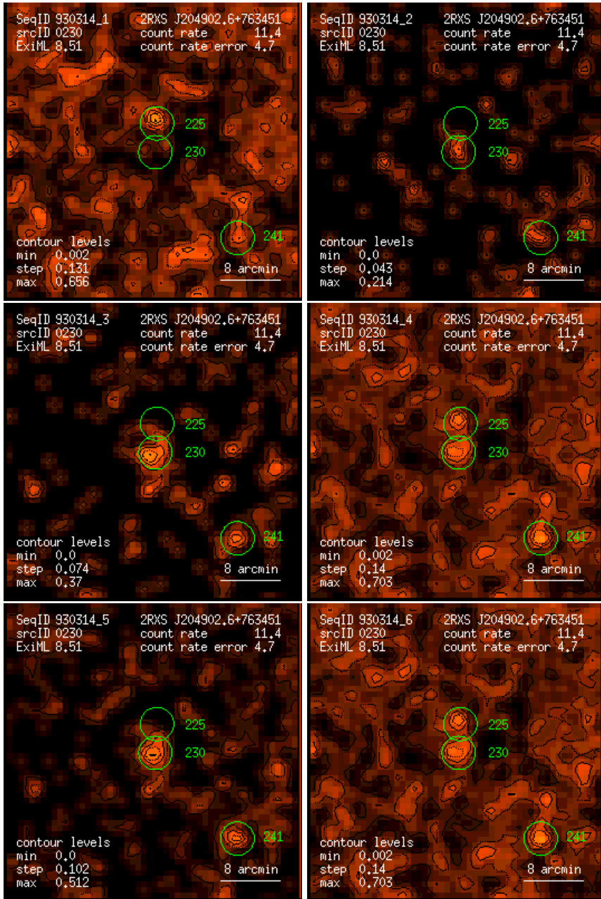
Figure 230: RASS 930314: detection 0230: band rate images, Gaussian filter: (1) PSPC channels 11 – 41, (2) 52 – 90, (3) 91 – 201, (4) 11 – 235, (5) 52 – 201, (6) 11 – 201. Broad band rates in counts/ks. Band rate contour levels in counts/ks/arcmin 2 .
