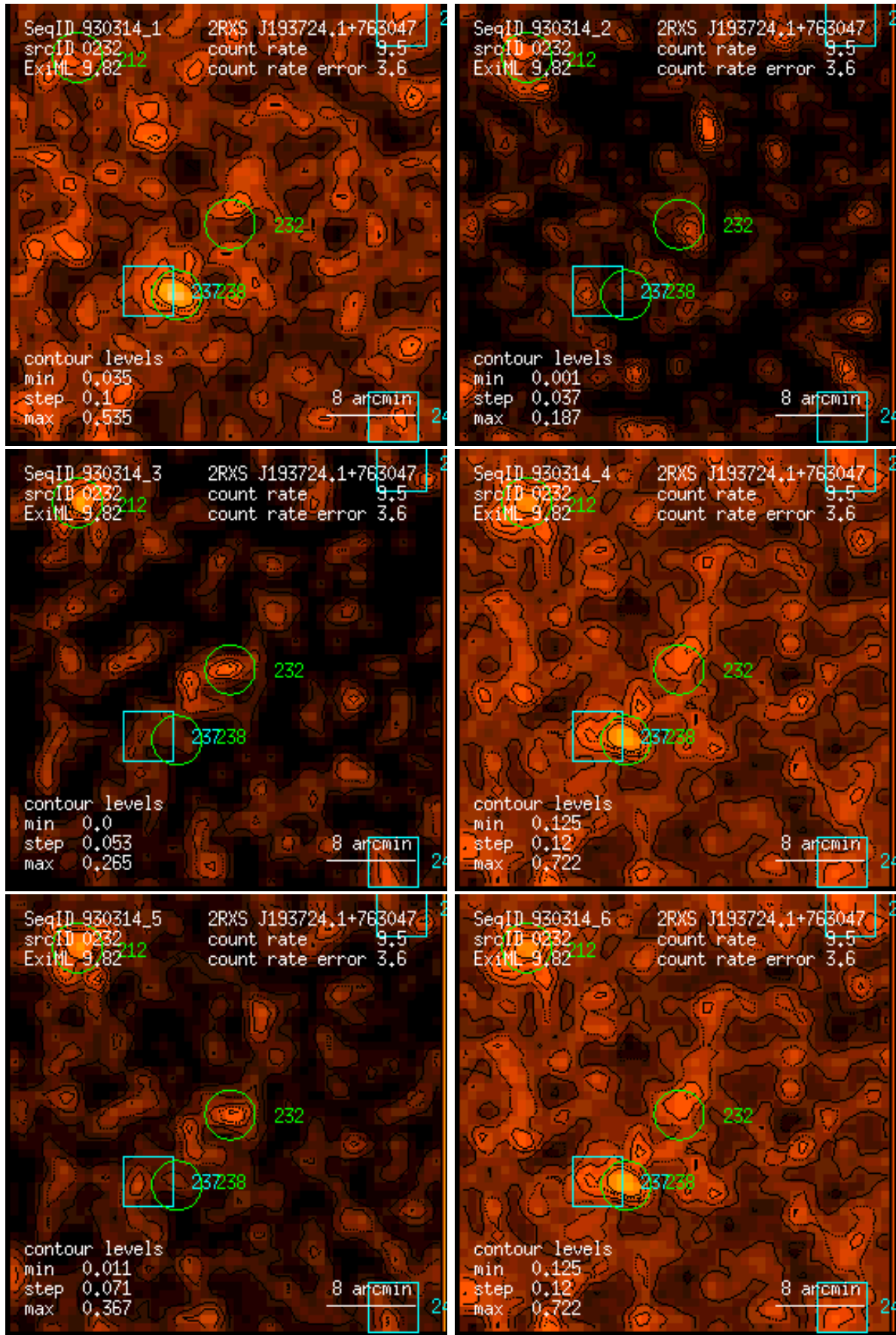
Figure 232: RASS 930314: detection 0232: band rate images, Gaussian filter: (1) PSPC channels 11 – 41, (2) 52 – 90, (3) 91 – 201, (4) 11 – 235, (5) 52 – 201, (6) 11 – 201. Broad band rates in counts/ks. Band rate contour levels in counts/ks/arcmin 2 .
