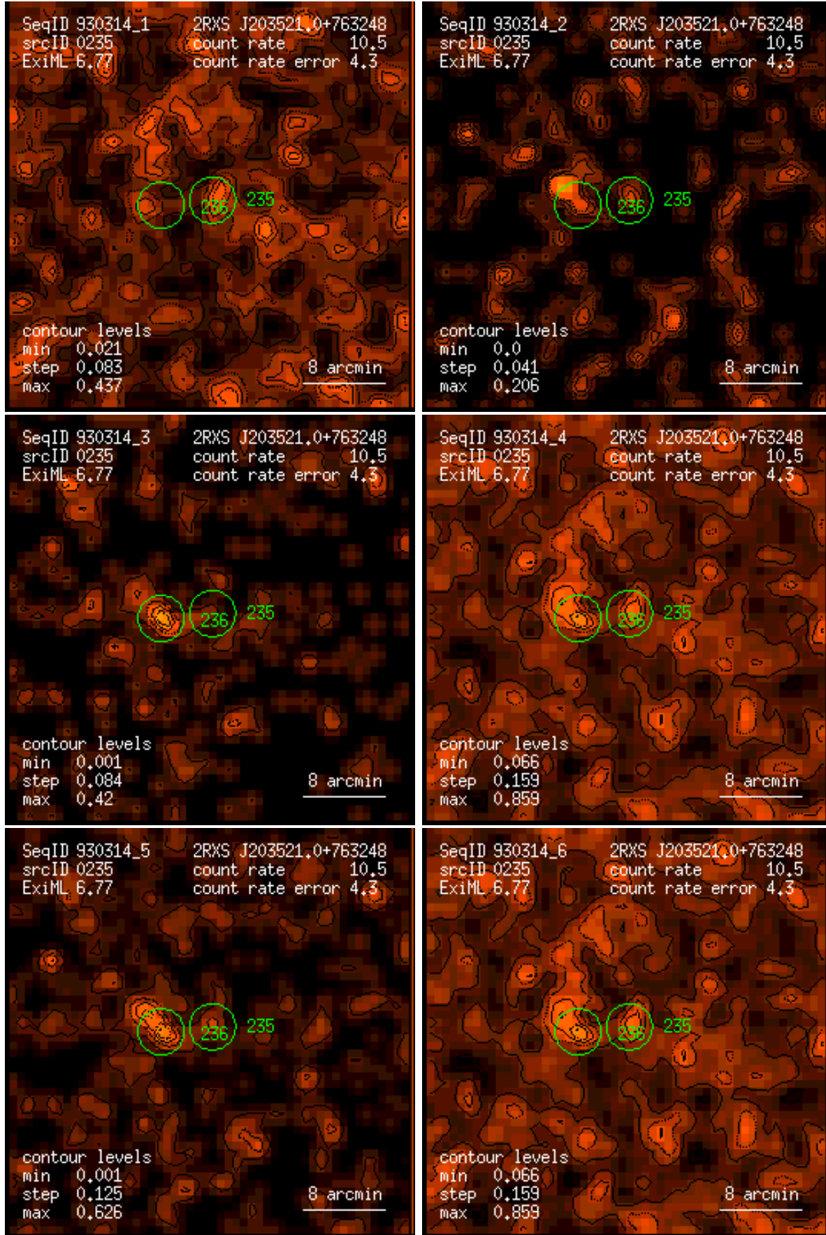
Figure 235: RASS 930314: detection 0235: band rate images, Gaussian filter: (1) PSPC channels 11 – 41, (2) 52 – 90, (3) 91 – 201, (4) 11 – 235, (5) 52 – 201, (6) 11 – 201. Broad band rates in counts/ks. Band rate contour levels in counts/ks/arcmin 2 .
