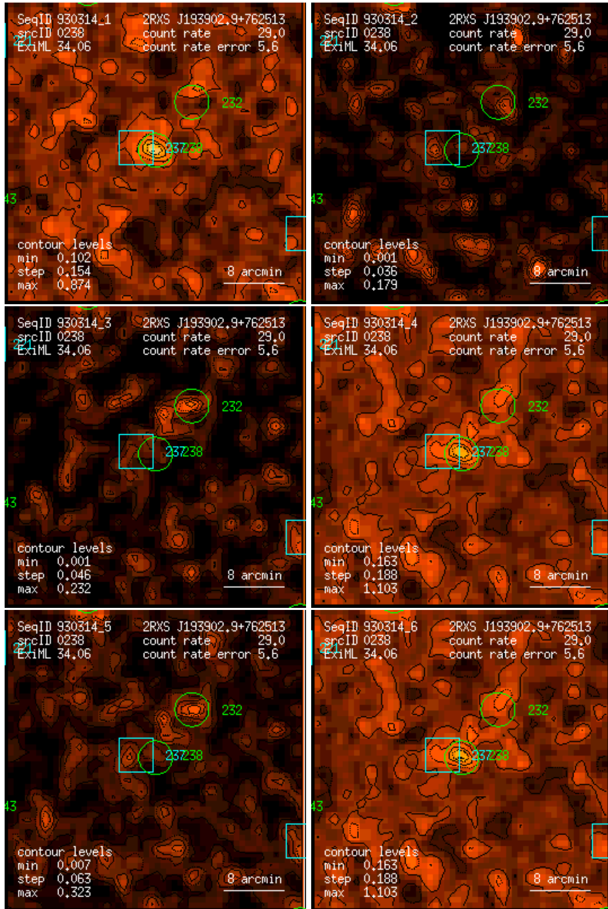
Figure 238: RASS 930314: detection 0238: band rate images, Gaussian filter: (1) PSPC channels 11 – 41, (2) 52 – 90, (3) 91 – 201, (4) 11 – 235, (5) 52 – 201, (6) 11 – 201. Broad band rates in counts/ks. Band rate contour levels in counts/ks/arcmin 2 .
