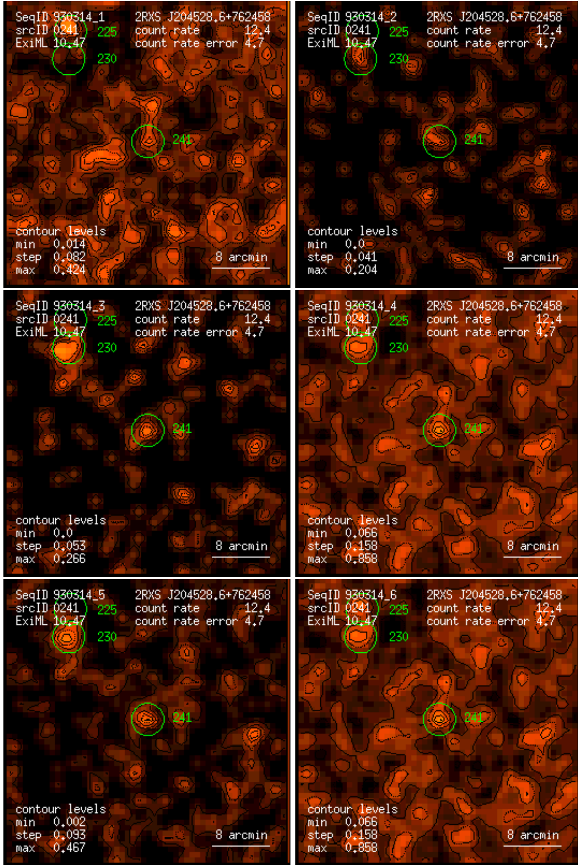
Figure 241: RASS 930314: detection 0241: band rate images, Gaussian filter: (1) PSPC channels 11 – 41, (2) 52 – 90, (3) 91 – 201, (4) 11 – 235, (5) 52 – 201, (6) 11 – 201. Broad band rates in counts/ks. Band rate contour levels in counts/ks/arcmin 2 .
