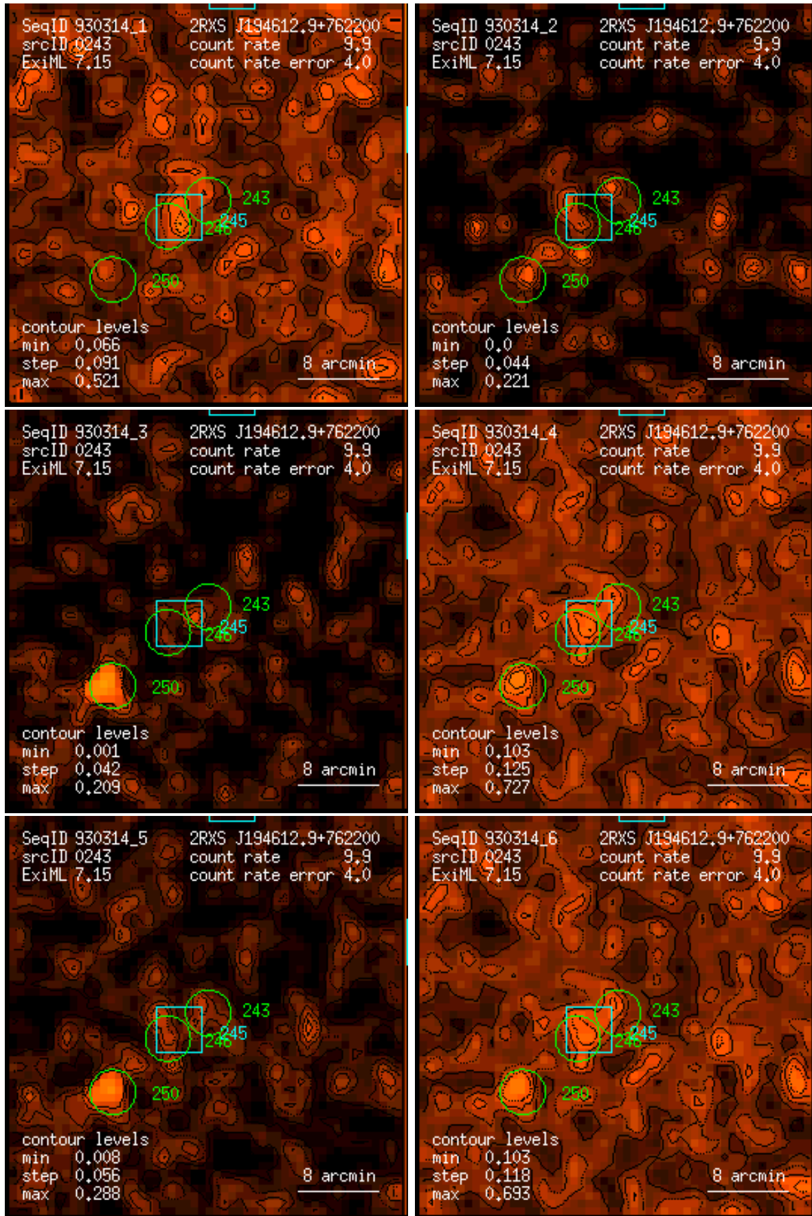
Figure 243: RASS 930314: detection 0243: band rate images, Gaussian filter: (1) PSPC channels 11 – 41, (2) 52 – 90, (3) 91 – 201, (4) 11 – 235, (5) 52 – 201, (6) 11 – 201. Broad band rates in counts/ks. Band rate contour levels in counts/ks/arcmin 2 .
