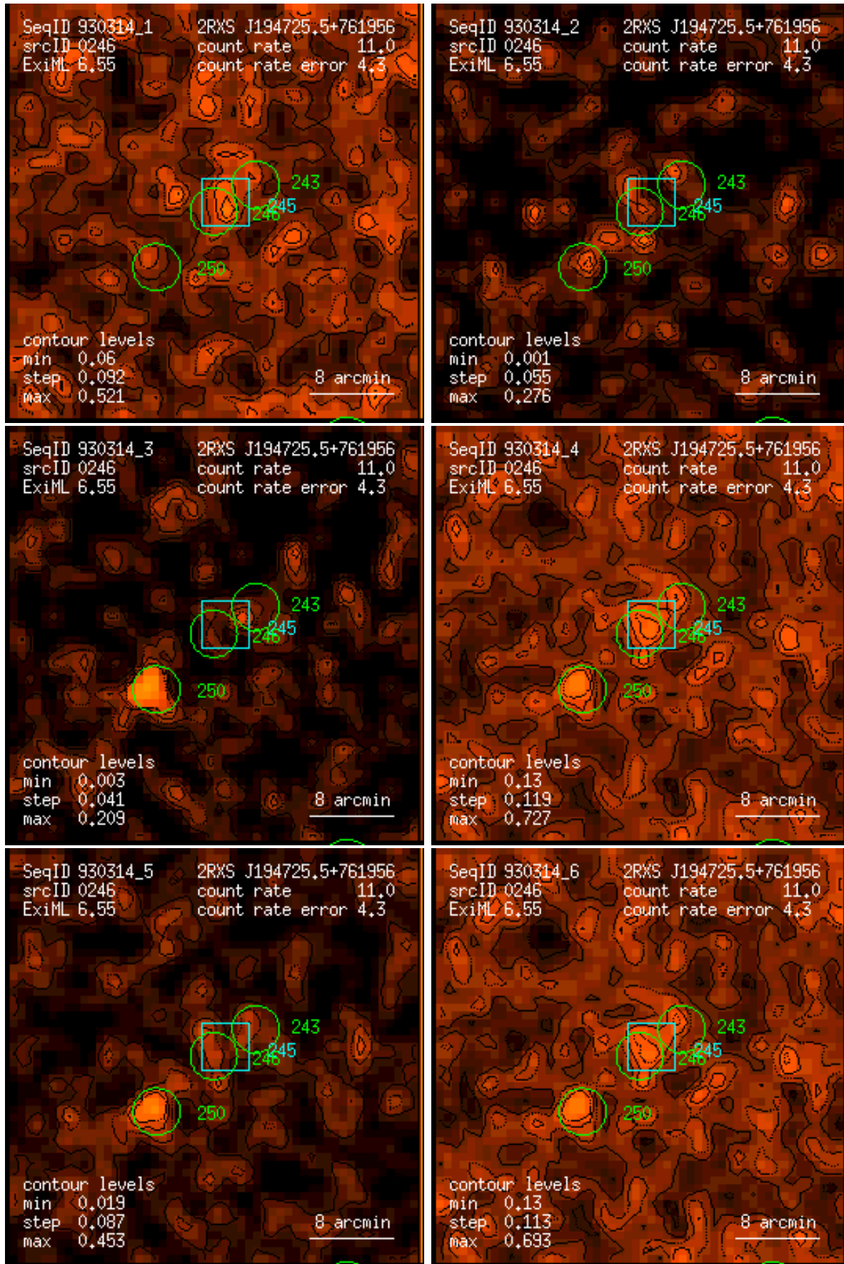
Figure 246: RASS 930314: detection 0246: band rate images, Gaussian filter: (1) PSPC channels 11 – 41, (2) 52 – 90, (3) 91 – 201, (4) 11 – 235, (5) 52 – 201, (6) 11 – 201. Broad band rates in counts/ks. Band rate contour levels in counts/ks/arcmin 2 .
