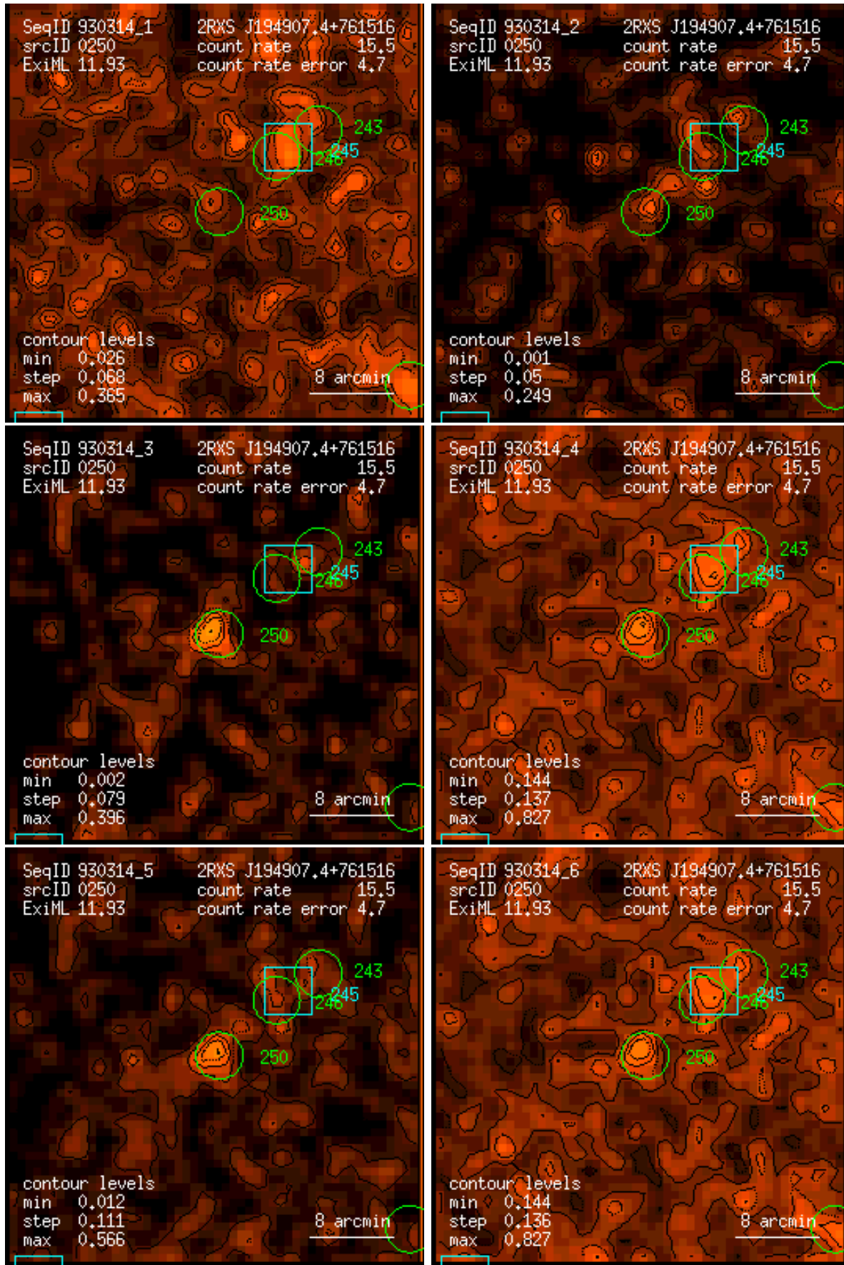
Figure 250: RASS 930314: detection 0250: band rate images, Gaussian filter: (1) PSPC channels 11 – 41, (2) 52 – 90, (3) 91 – 201, (4) 11 – 235, (5) 52 – 201, (6) 11 – 201. Broad band rates in counts/ks. Band rate contour levels in counts/ks/arcmin 2 .
