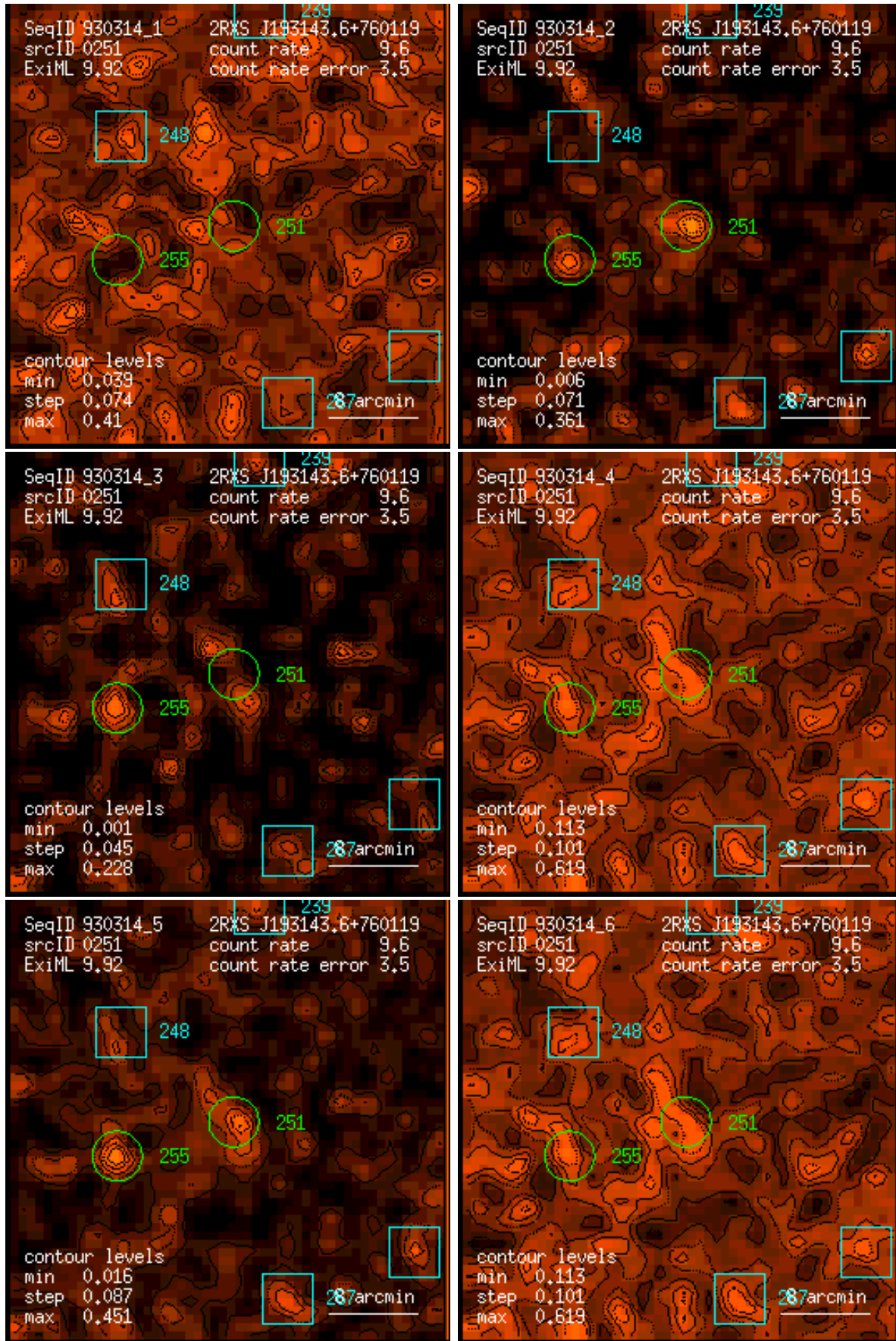
Figure 251: RASS 930314: detection 0251: band rate images, Gaussian filter: (1) PSPC channels 11 – 41, (2) 52 – 90, (3) 91 – 201, (4) 11 – 235, (5) 52 – 201, (6) 11 – 201. Broad band rates in counts/ks. Band rate contour levels in counts/ks/arcmin 2 .
