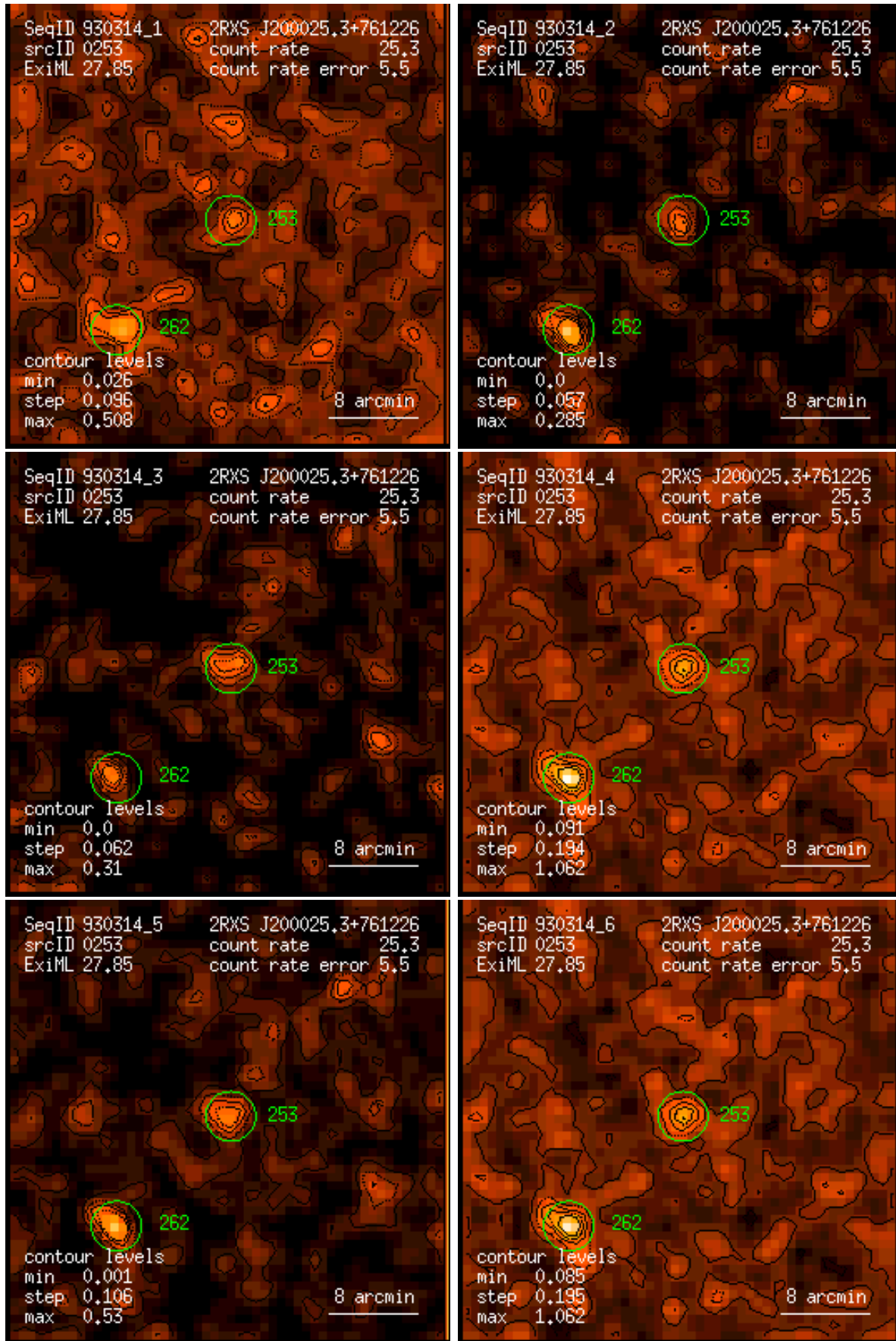
Figure 253: RASS 930314: detection 0253: band rate images, Gaussian filter: (1) PSPC channels 11 – 41, (2) 52 – 90, (3) 91 – 201, (4) 11 – 235, (5) 52 – 201, (6) 11 – 201. Broad band rates in counts/ks. Band rate contour levels in counts/ks/arcmin 2 .
