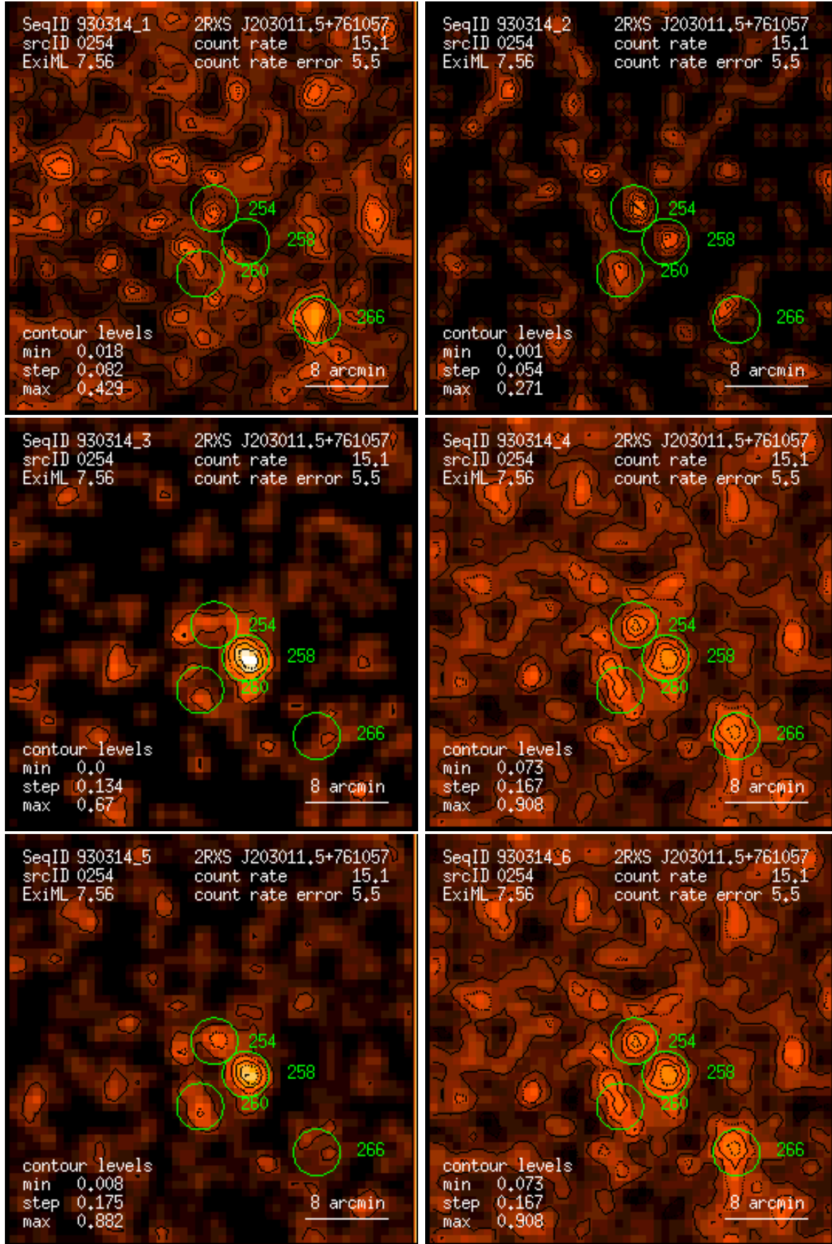
Figure 254: RASS 930314: detection 0254: band rate images, Gaussian filter: (1) PSPC channels 11 – 41, (2) 52 – 90, (3) 91 – 201, (4) 11 – 235, (5) 52 – 201, (6) 11 – 201. Broad band rates in counts/ks. Band rate contour levels in counts/ks/arcmin 2 .
