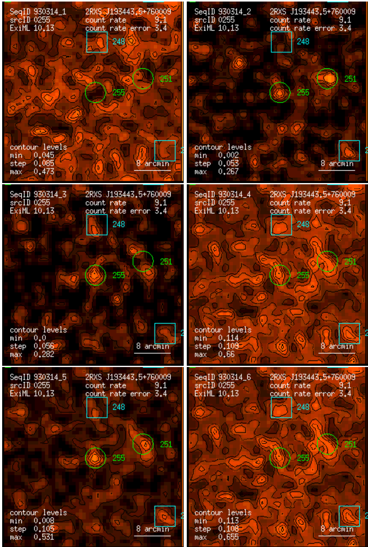
Figure 255: RASS 930314: detection 0255: band rate images, Gaussian filter: (1) PSPC channels 11 – 41, (2) 52 – 90, (3) 91 – 201, (4) 11 – 235, (5) 52 – 201, (6) 11 – 201. Broad band rates in counts/ks. Band rate contour levels in counts/ks/arcmin 2 .
