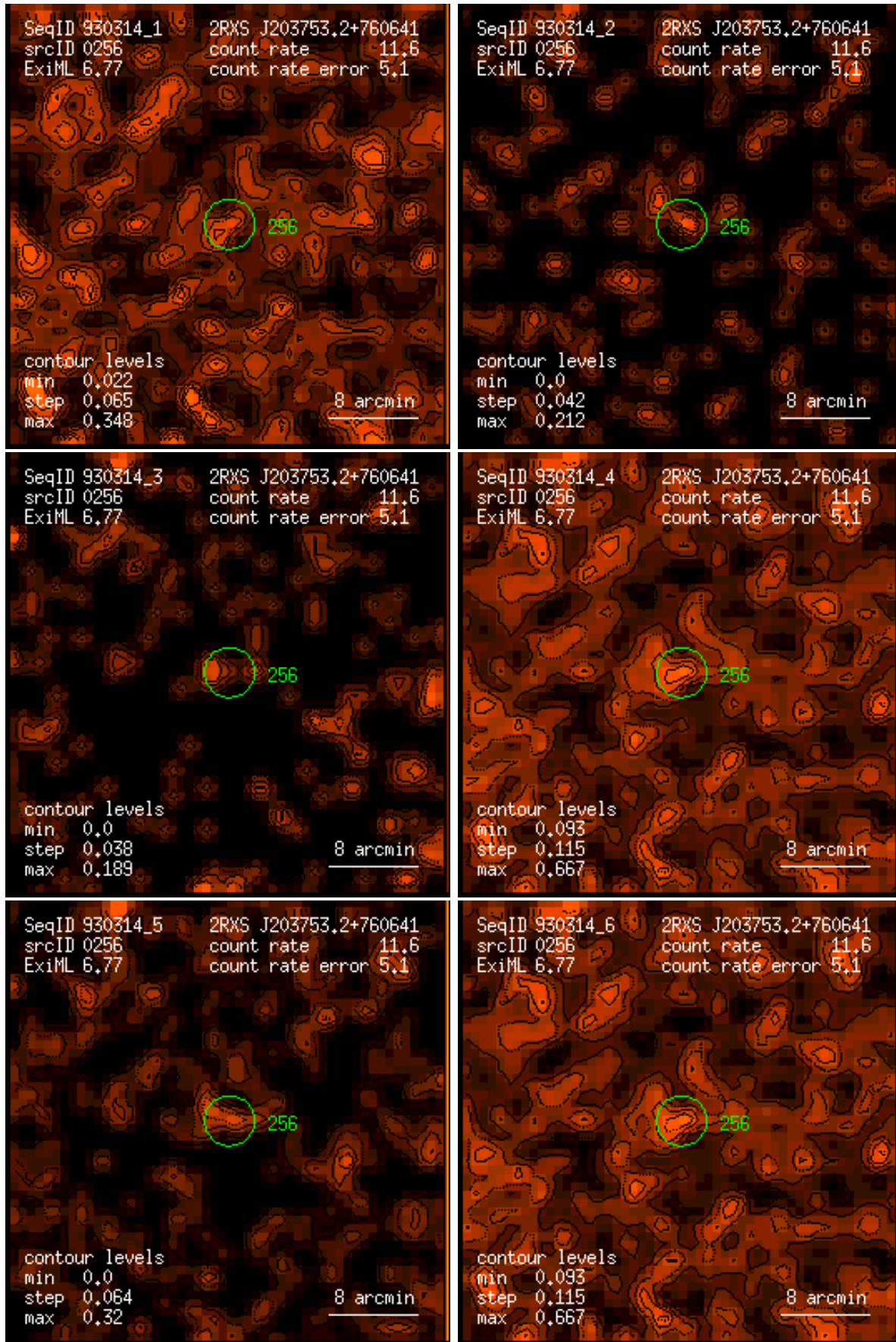
Figure 256: RASS 930314: detection 0256: band rate images, Gaussian filter: (1) PSPC channels 11 – 41, (2) 52 – 90, (3) 91 – 201, (4) 11 – 235, (5) 52 – 201, (6) 11 – 201. Broad band rates in counts/ks. Band rate contour levels in counts/ks/arcmin 2 .
