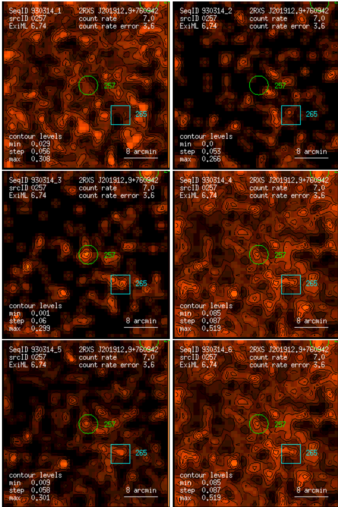
Figure 257: RASS 930314: detection 0257: band rate images, Gaussian filter: (1) PSPC channels 11 – 41, (2) 52 – 90, (3) 91 – 201, (4) 11 – 235, (5) 52 – 201, (6) 11 – 201. Broad band rates in counts/ks. Band rate contour levels in counts/ks/arcmin 2 .
