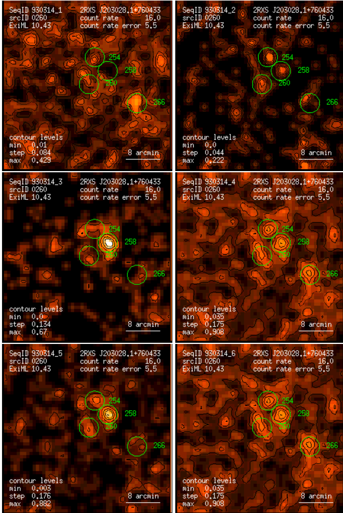
Figure 260: RASS 930314: detection 0260: band rate images, Gaussian filter: (1) PSPC channels 11 – 41, (2) 52 – 90, (3) 91 – 201, (4) 11 – 235, (5) 52 – 201, (6) 11 – 201. Broad band rates in counts/ks. Band rate contour levels in counts/ks/arcmin 2 .
