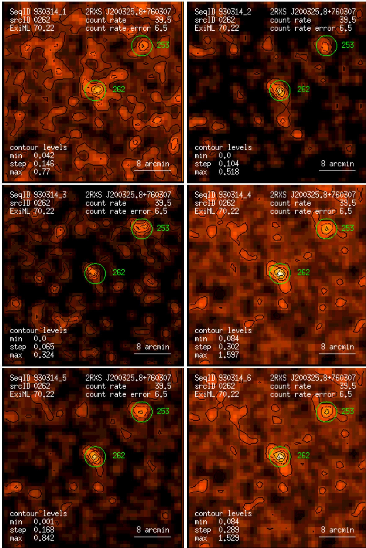
Figure 262: RASS 930314: detection 0262: band rate images, Gaussian filter: (1) PSPC channels 11 – 41, (2) 52 – 90, (3) 91 – 201, (4) 11 – 235, (5) 52 – 201, (6) 11 – 201. Broad band rates in counts/ks. Band rate contour levels in counts/ks/arcmin 2 .
