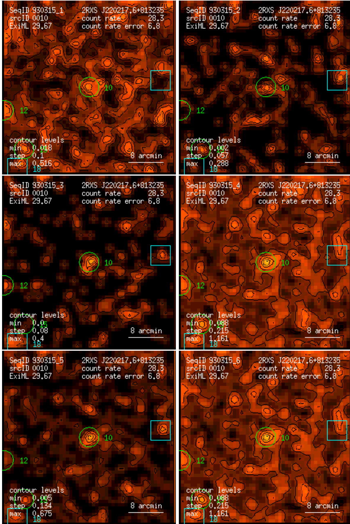
Figure 10: RASS 930315: detection 0010: band rate images, Gaussian filter: (1) PSPC channels 11 – 41, (2) 52 – 90, (3) 91 – 201, (4) 11 – 235, (5) 52 – 201, (6) 11 – 201. Broad band rates in counts/ks. Band rate contour levels in counts/ks/arcmin 2 .
