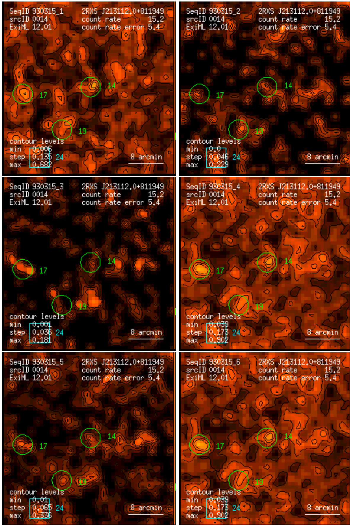
Figure 14: RASS 930315: detection 0014: band rate images, Gaussian filter: (1) PSPC channels 11 – 41, (2) 52 – 90, (3) 91 – 201, (4) 11 – 235, (5) 52 – 201, (6) 11 – 201. Broad band rates in counts/ks. Band rate contour levels in counts/ks/arcmin 2 .
