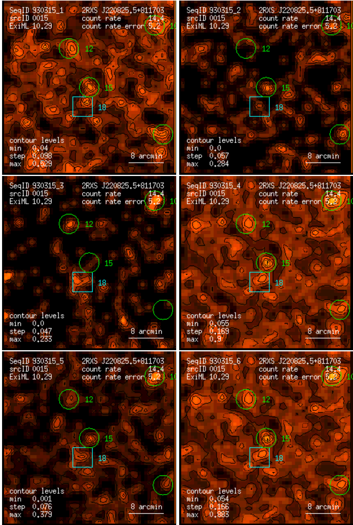
Figure 15: RASS 930315: detection 0015: band rate images, Gaussian filter: (1) PSPC channels 11 – 41, (2) 52 – 90, (3) 91 – 201, (4) 11 – 235, (5) 52 – 201, (6) 11 – 201. Broad band rates in counts/ks. Band rate contour levels in counts/ks/arcmin 2 .
