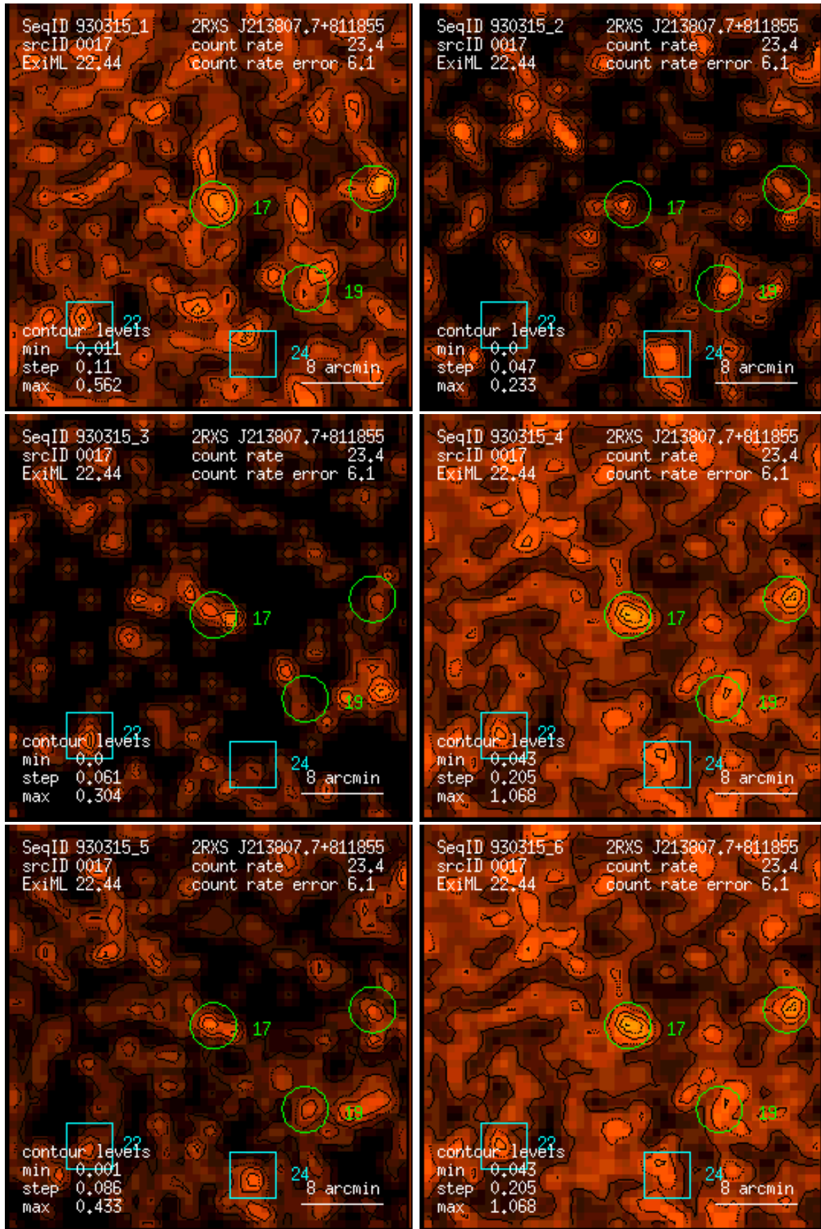
Figure 17: RASS 930315: detection 0017: band rate images, Gaussian filter: (1) PSPC channels 11 – 41, (2) 52 – 90, (3) 91 – 201, (4) 11 – 235, (5) 52 – 201, (6) 11 – 201. Broad band rates in counts/ks. Band rate contour levels in counts/ks/arcmin 2 .
