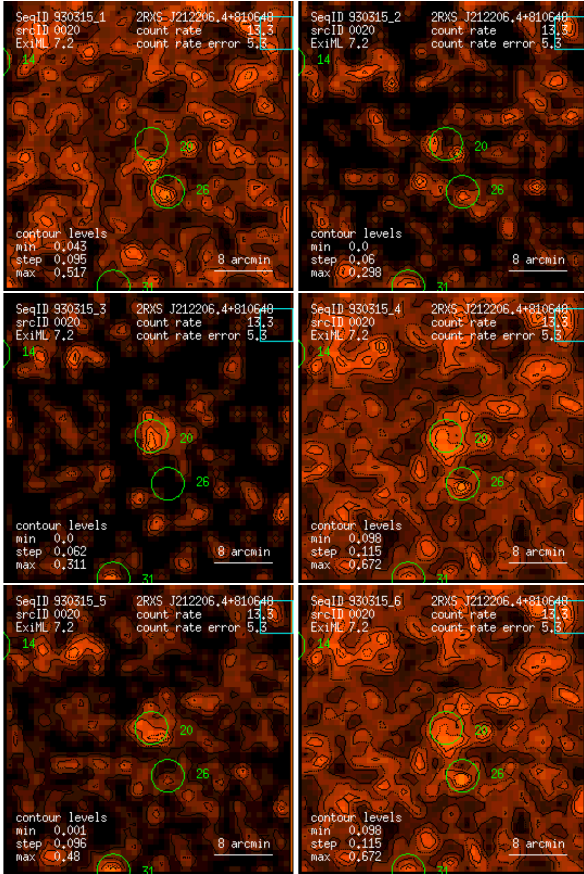
Figure 20: RASS 930315: detection 0020: band rate images, Gaussian filter: (1) PSPC channels 11 – 41, (2) 52 – 90, (3) 91 – 201, (4) 11 – 235, (5) 52 – 201, (6) 11 – 201. Broad band rates in counts/ks. Band rate contour levels in counts/ks/arcmin 2 .
