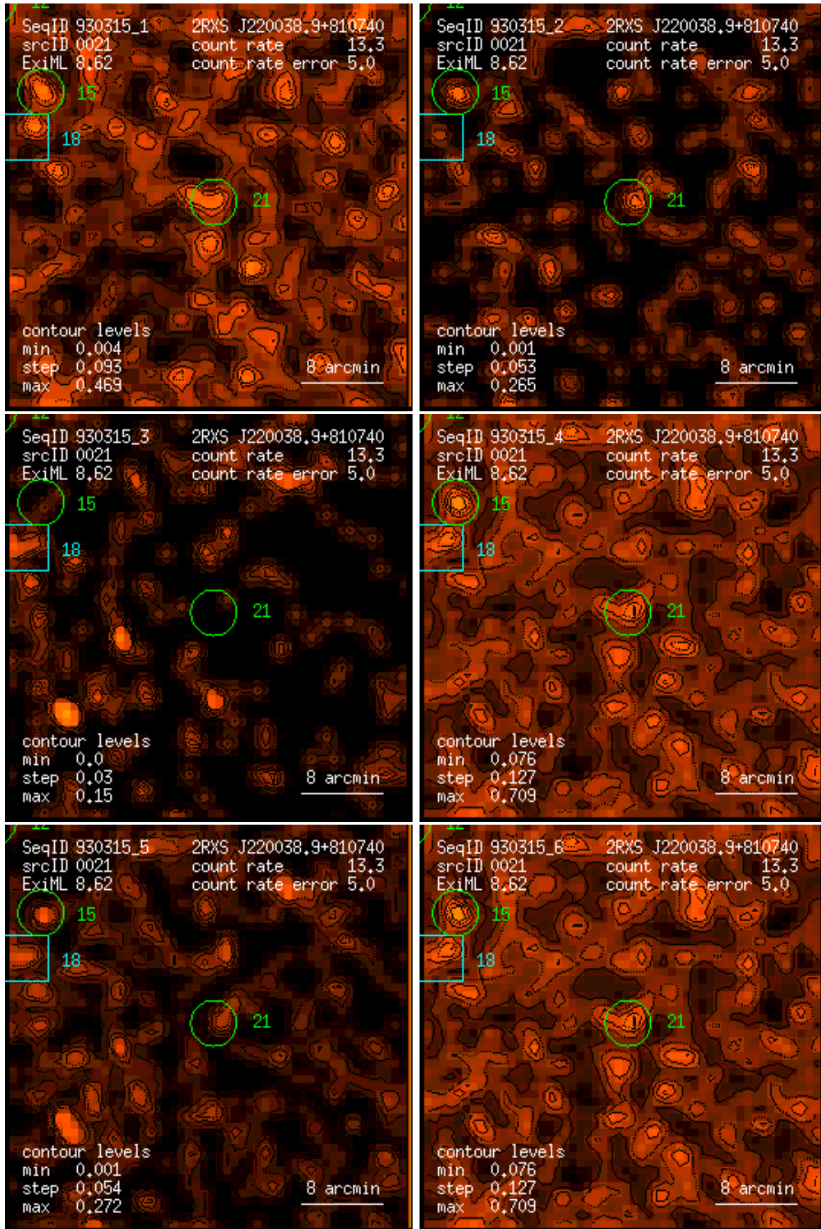
Figure 21: RASS 930315: detection 0021: band rate images, Gaussian filter: (1) PSPC channels 11 – 41, (2) 52 – 90, (3) 91 – 201, (4) 11 – 235, (5) 52 – 201, (6) 11 – 201. Broad band rates in counts/ks. Band rate contour levels in counts/ks/arcmin 2 .
