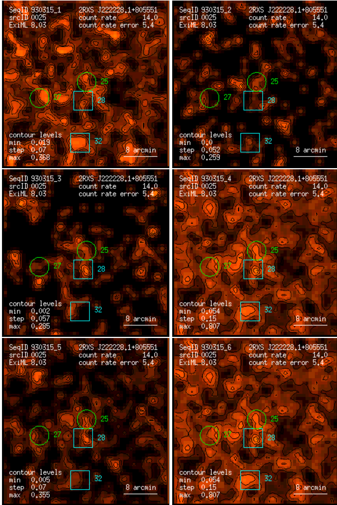
Figure 25: RASS 930315: detection 0025: band rate images, Gaussian filter: (1) PSPC channels 11 – 41, (2) 52 – 90, (3) 91 – 201, (4) 11 – 235, (5) 52 – 201, (6) 11 – 201. Broad band rates in counts/ks. Band rate contour levels in counts/ks/arcmin 2 .
