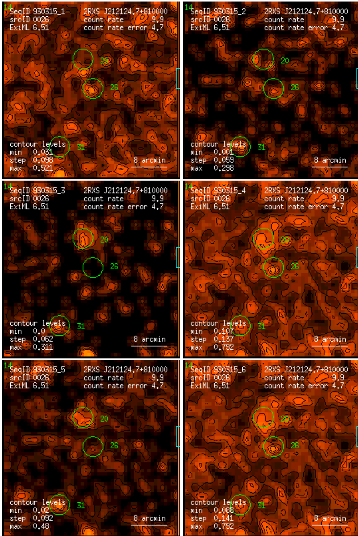
Figure 26: RASS 930315: detection 0026: band rate images, Gaussian filter: (1) PSPC channels 11 – 41, (2) 52 – 90, (3) 91 – 201, (4) 11 – 235, (5) 52 – 201, (6) 11 – 201. Broad band rates in counts/ks. Band rate contour levels in counts/ks/arcmin 2 .
