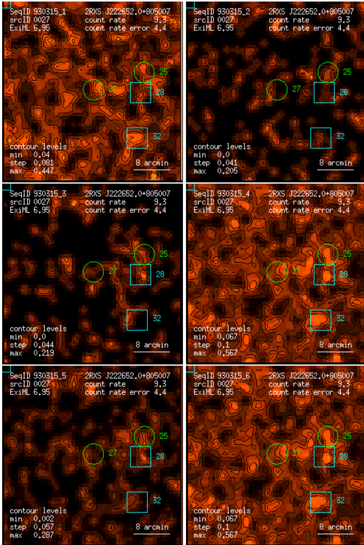
Figure 27: RASS 930315: detection 0027: band rate images, Gaussian filter: (1) PSPC channels 11 – 41, (2) 52 – 90, (3) 91 – 201, (4) 11 – 235, (5) 52 – 201, (6) 11 – 201. Broad band rates in counts/ks. Band rate contour levels in counts/ks/arcmin 2 .
