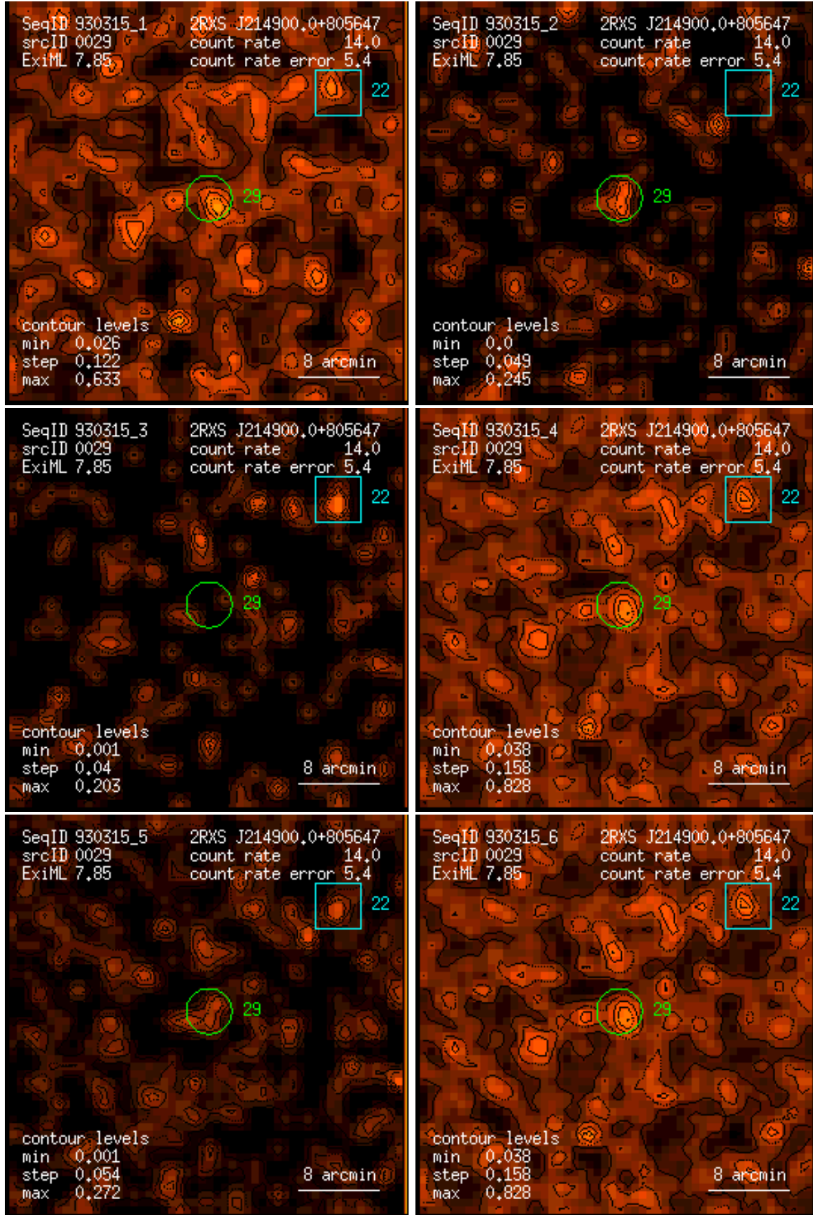
Figure 29: RASS 930315: detection 0029: band rate images, Gaussian filter: (1) PSPC channels 11 – 41, (2) 52 – 90, (3) 91 – 201, (4) 11 – 235, (5) 52 – 201, (6) 11 – 201. Broad band rates in counts/ks. Band rate contour levels in counts/ks/arcmin 2 .
