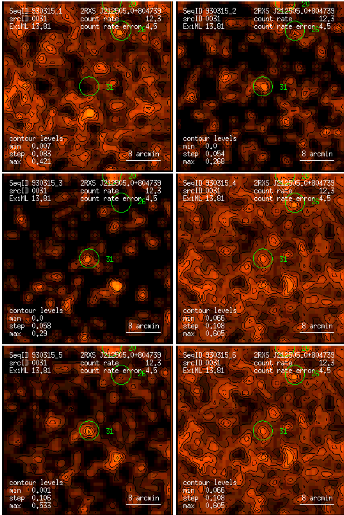
Figure 31: RASS 930315: detection 0031: band rate images, Gaussian filter: (1) PSPC channels 11 – 41, (2) 52 – 90, (3) 91 – 201, (4) 11 – 235, (5) 52 – 201, (6) 11 – 201. Broad band rates in counts/ks. Band rate contour levels in counts/ks/arcmin 2 .
