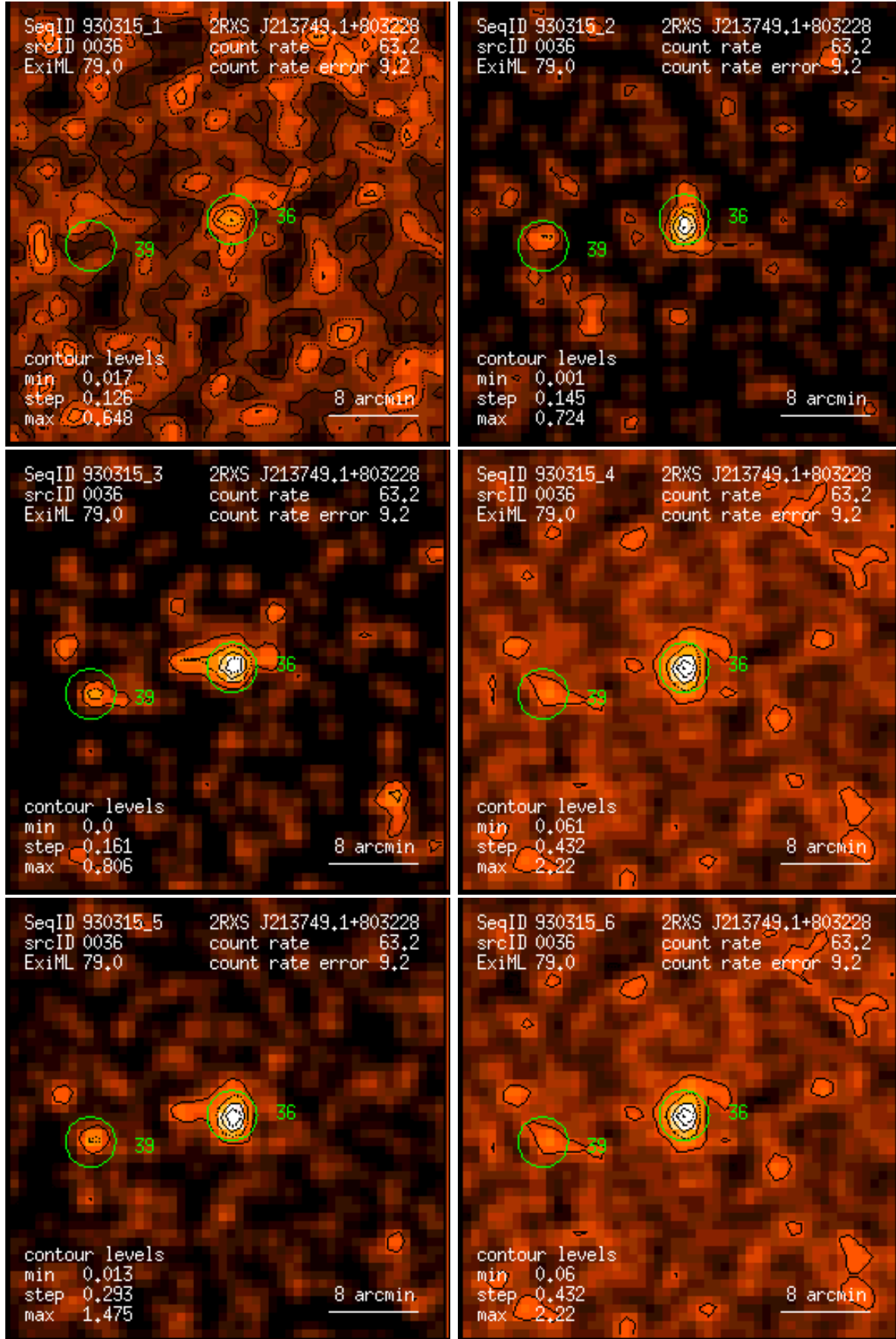
Figure 36: RASS 930315: detection 0036: band rate images, Gaussian filter: (1) PSPC channels 11 – 41, (2) 52 – 90, (3) 91 – 201, (4) 11 – 235, (5) 52 – 201, (6) 11 – 201. Broad band rates in counts/ks. Band rate contour levels in counts/ks/arcmin 2 .
