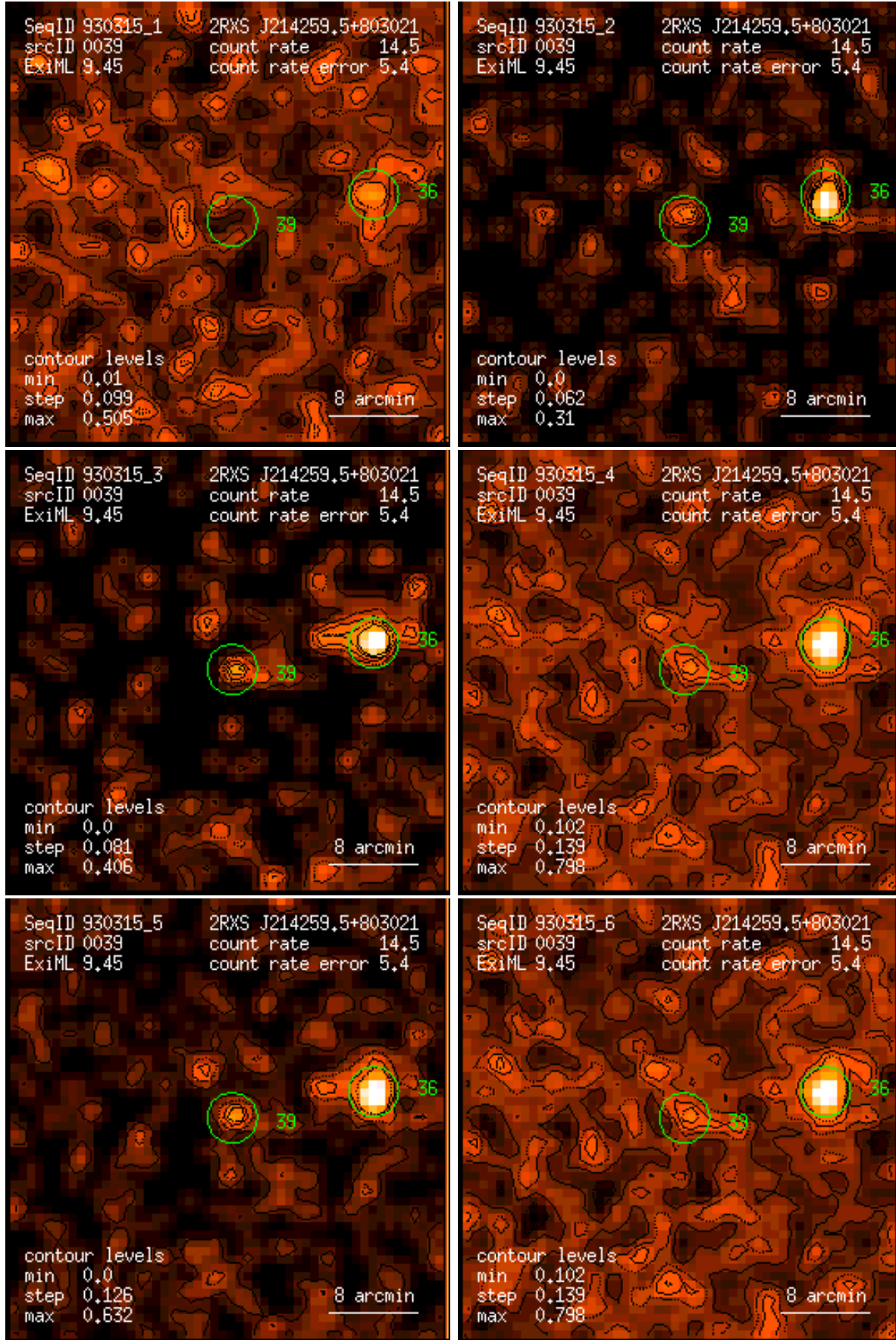
Figure 39: RASS 930315: detection 0039: band rate images, Gaussian filter: (1) PSPC channels 11 – 41, (2) 52 – 90, (3) 91 – 201, (4) 11 – 235, (5) 52 – 201, (6) 11 – 201. Broad band rates in counts/ks. Band rate contour levels in counts/ks/arcmin 2 .
