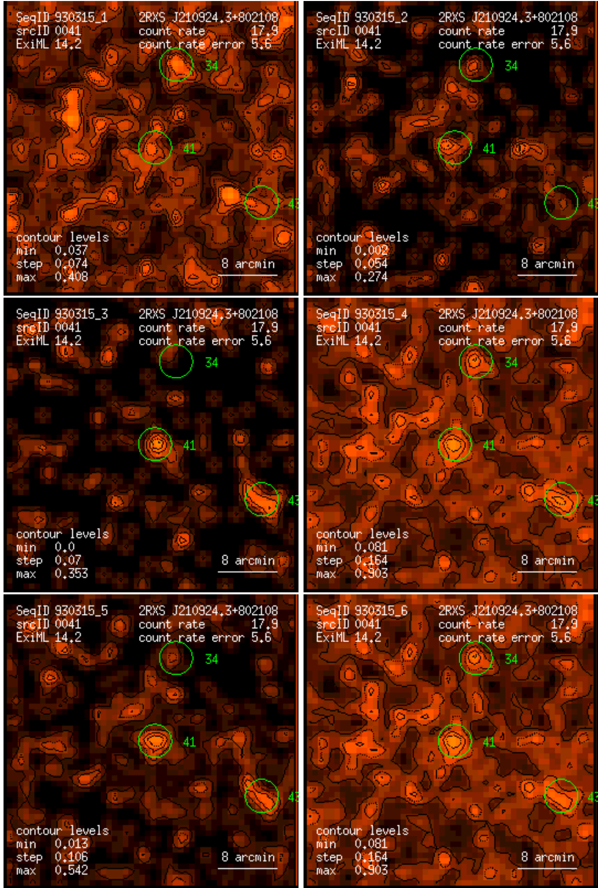
Figure 41: RASS 930315: detection 0041: band rate images, Gaussian filter: (1) PSPC channels 11 – 41, (2) 52 – 90, (3) 91 – 201, (4) 11 – 235, (5) 52 – 201, (6) 11 – 201. Broad band rates in counts/ks. Band rate contour levels in counts/ks/arcmin 2 .
