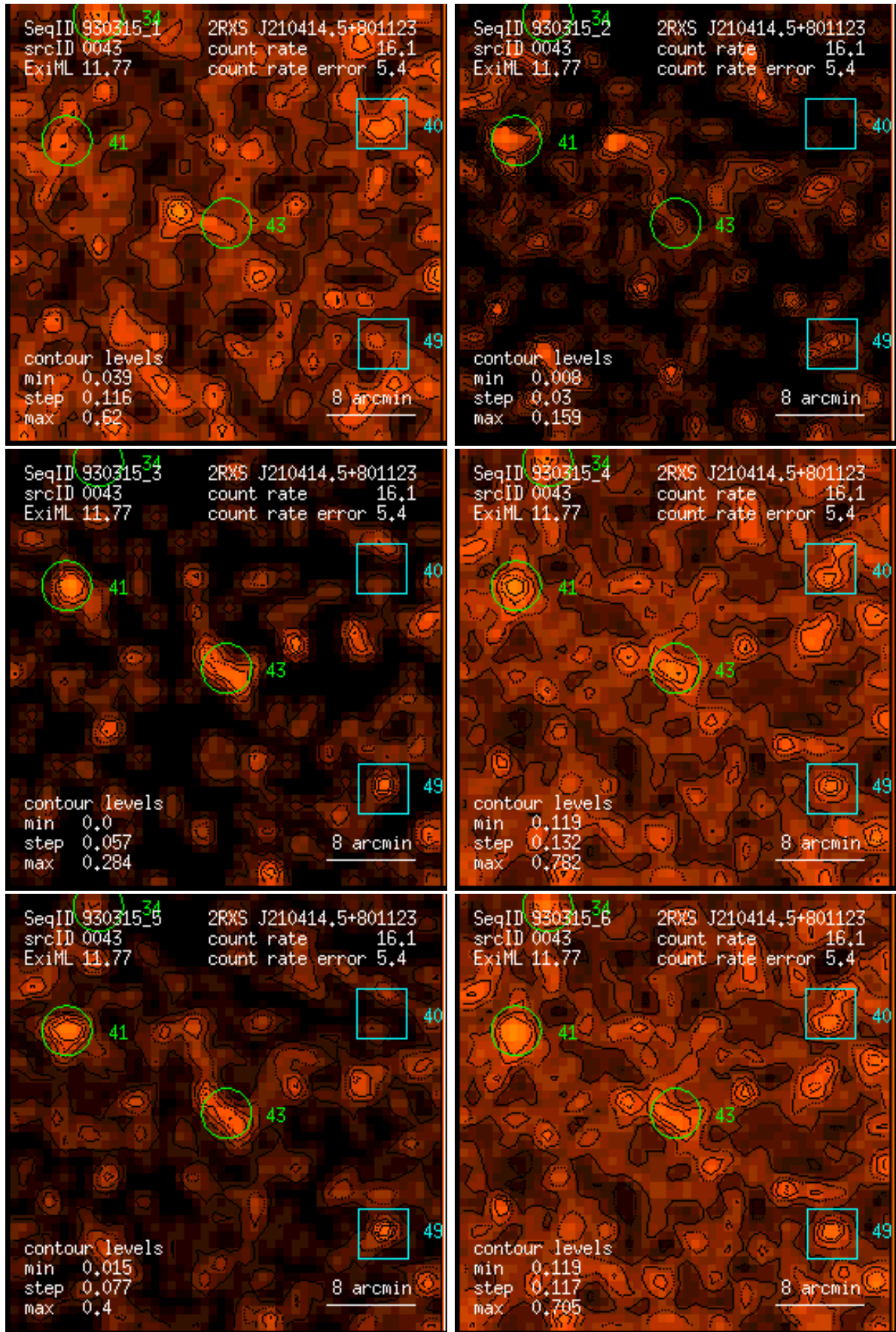
Figure 43: RASS 930315: detection 0043: band rate images, Gaussian filter: (1) PSPC channels 11 – 41, (2) 52 – 90, (3) 91 – 201, (4) 11 – 235, (5) 52 – 201, (6) 11 – 201. Broad band rates in counts/ks. Band rate contour levels in counts/ks/arcmin 2 .
