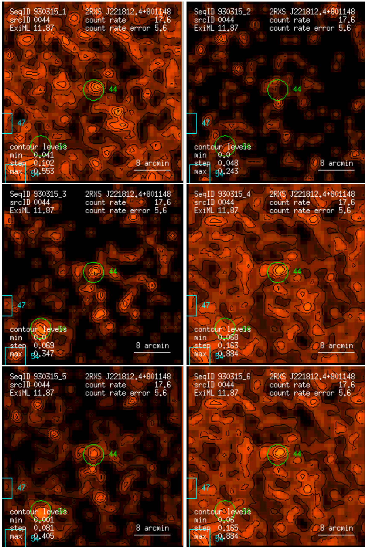
Figure 44: RASS 930315: detection 0044: band rate images, Gaussian filter: (1) PSPC channels 11 – 41, (2) 52 – 90, (3) 91 – 201, (4) 11 – 235, (5) 52 – 201, (6) 11 – 201. Broad band rates in counts/ks. Band rate contour levels in counts/ks/arcmin 2 .
