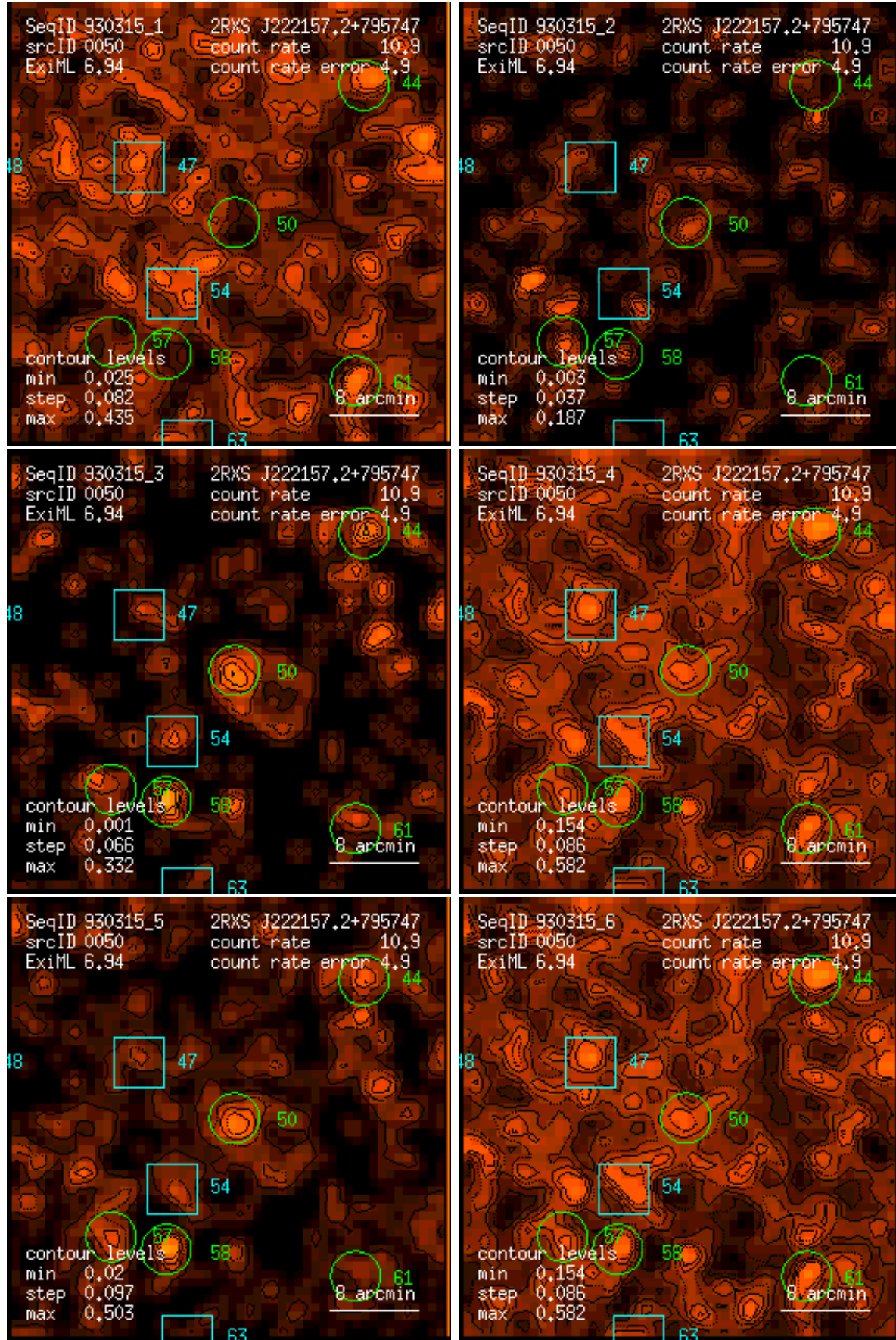
Figure 50: RASS 930315: detection 0050: band rate images, Gaussian filter: (1) PSPC channels 11 – 41, (2) 52 – 90, (3) 91 – 201, (4) 11 – 235, (5) 52 – 201, (6) 11 – 201. Broad band rates in counts/ks. Band rate contour levels in counts/ks/arcmin 2 .
