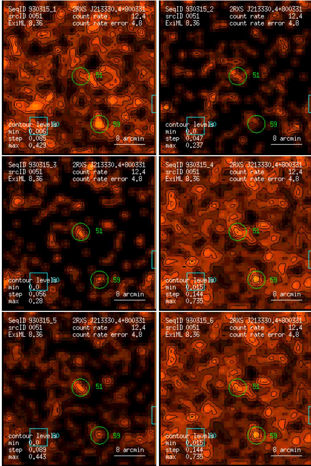
Figure 51: RASS 930315: detection 0051: band rate images, Gaussian filter: (1) PSPC channels 11 – 41, (2) 52 – 90, (3) 91 – 201, (4) 11 – 235, (5) 52 – 201, (6) 11 – 201. Broad band rates in counts/ks. Band rate contour levels in counts/ks/arcmin 2 .
