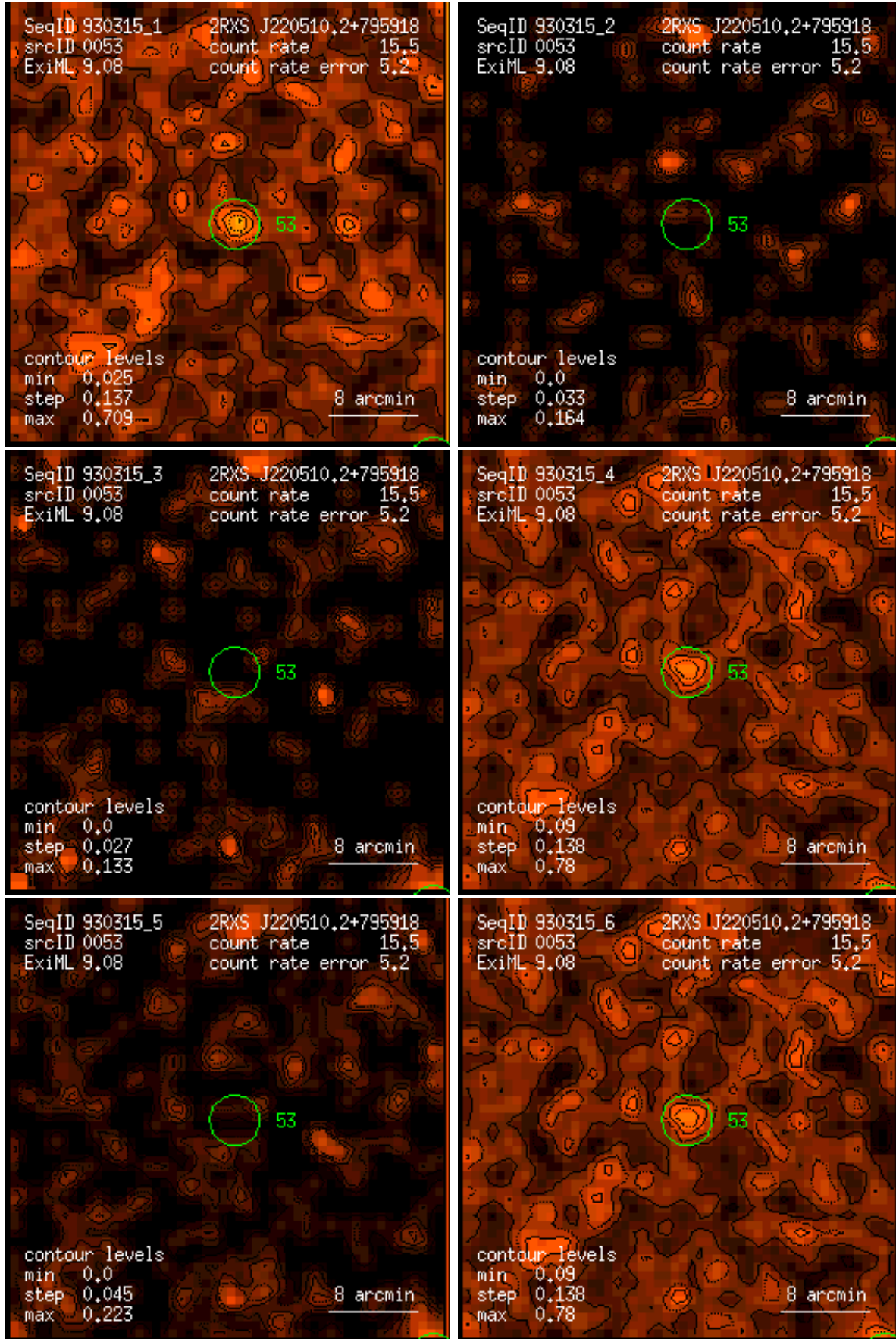
Figure 53: RASS 930315: detection 0053: band rate images, Gaussian filter: (1) PSPC channels 11 – 41, (2) 52 – 90, (3) 91 – 201, (4) 11 – 235, (5) 52 – 201, (6) 11 – 201. Broad band rates in counts/ks. Band rate contour levels in counts/ks/arcmin 2 .
