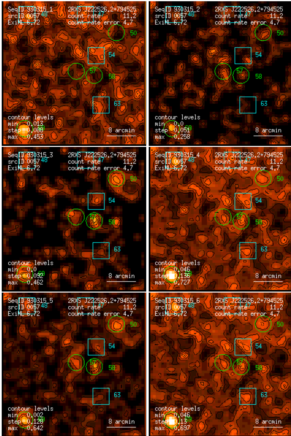
Figure 57: RASS 930315: detection 0057: band rate images, Gaussian filter: (1) PSPC channels 11 – 41, (2) 52 – 90, (3) 91 – 201, (4) 11 – 235, (5) 52 – 201, (6) 11 – 201. Broad band rates in counts/ks. Band rate contour levels in counts/ks/arcmin 2 .
