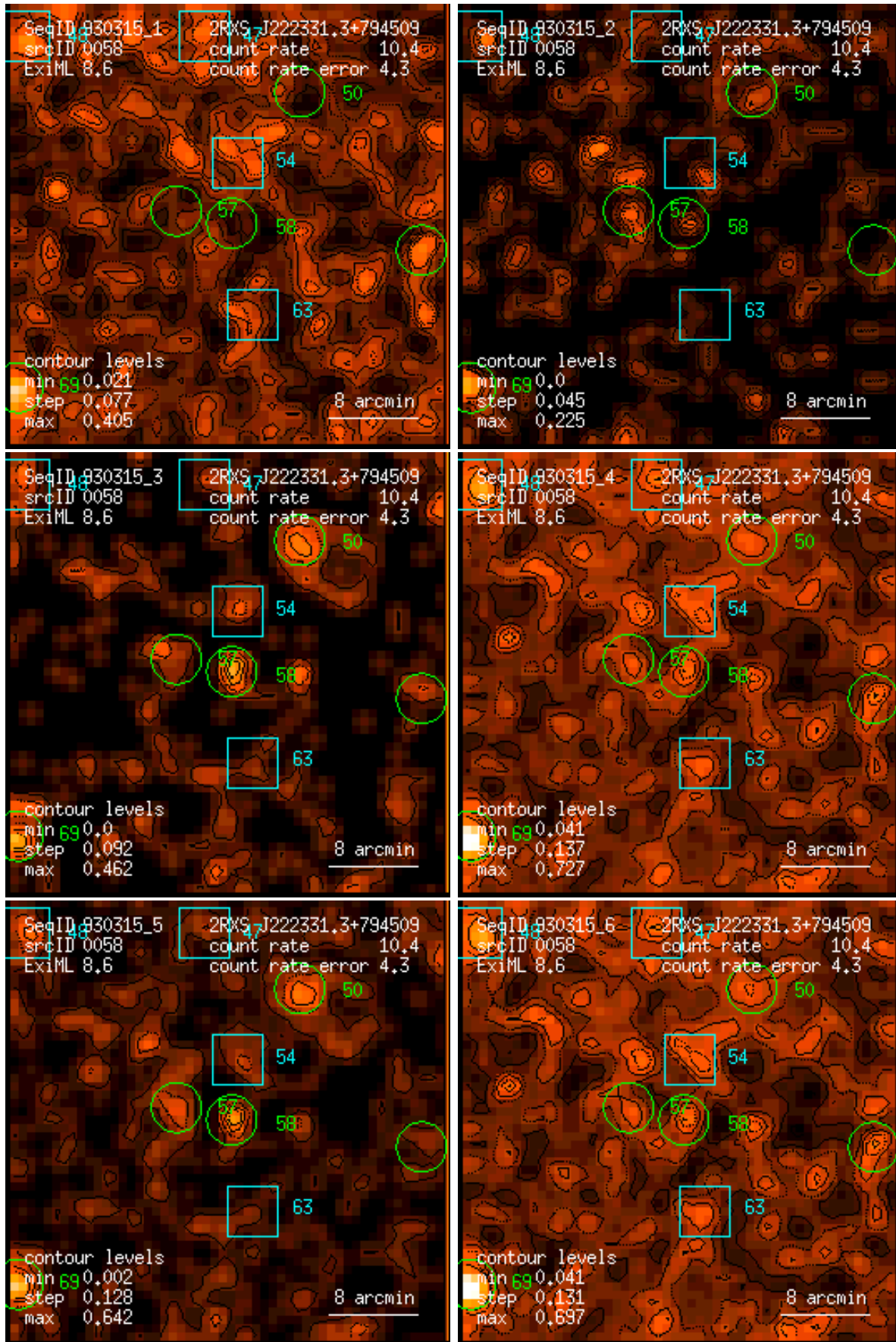
Figure 58: RASS 930315: detection 0058: band rate images, Gaussian filter: (1) PSPC channels 11 – 41, (2) 52 – 90, (3) 91 – 201, (4) 11 – 235, (5) 52 – 201, (6) 11 – 201. Broad band rates in counts/ks. Band rate contour levels in counts/ks/arcmin 2 .
