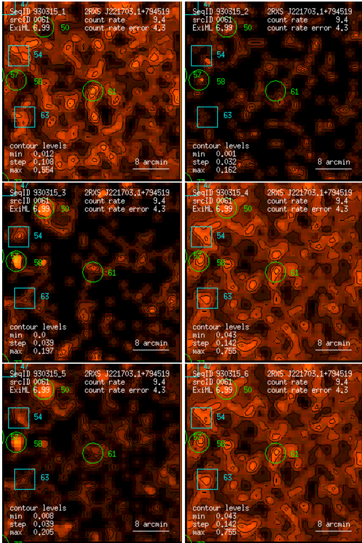
Figure 61: RASS 930315: detection 0061: band rate images, Gaussian filter: (1) PSPC channels 11 – 41, (2) 52 – 90, (3) 91 – 201, (4) 11 – 235, (5) 52 – 201, (6) 11 – 201. Broad band rates in counts/ks. Band rate contour levels in counts/ks/arcmin 2 .
