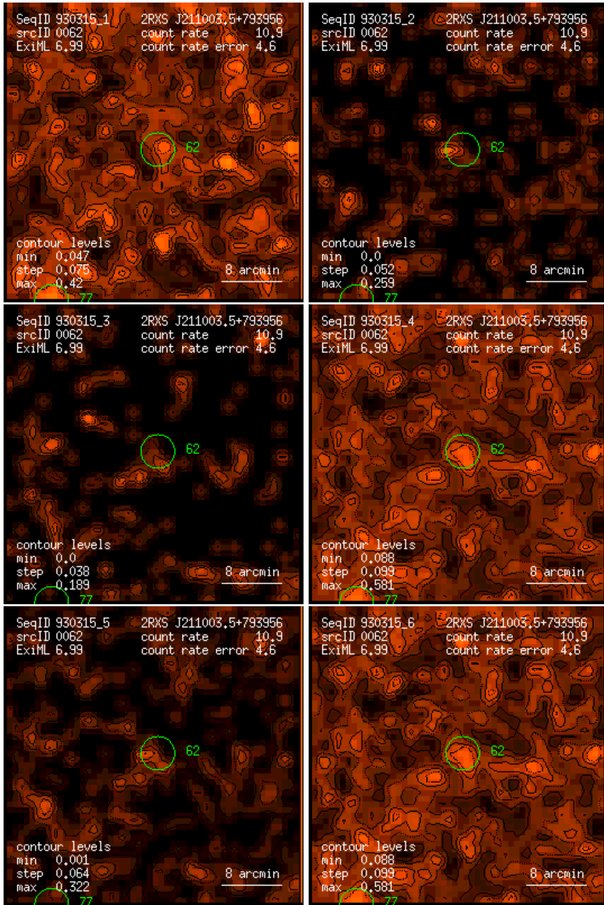
Figure 62: RASS 930315: detection 0062: band rate images, Gaussian filter: (1) PSPC channels 11 – 41, (2) 52 – 90, (3) 91 – 201, (4) 11 – 235, (5) 52 – 201, (6) 11 – 201. Broad band rates in counts/ks. Band rate contour levels in counts/ks/arcmin 2 .
