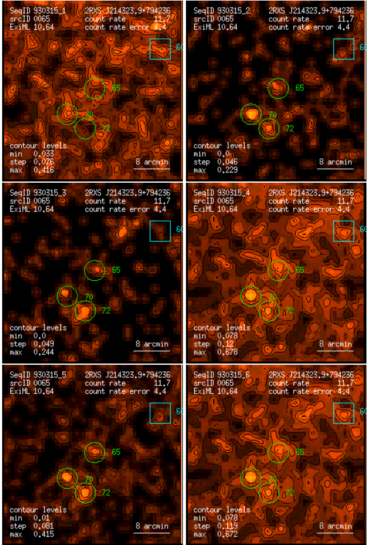
Figure 65: RASS 930315: detection 0065: band rate images, Gaussian filter: (1) PSPC channels 11 – 41, (2) 52 – 90, (3) 91 – 201, (4) 11 – 235, (5) 52 – 201, (6) 11 – 201. Broad band rates in counts/ks. Band rate contour levels in counts/ks/arcmin 2 .
