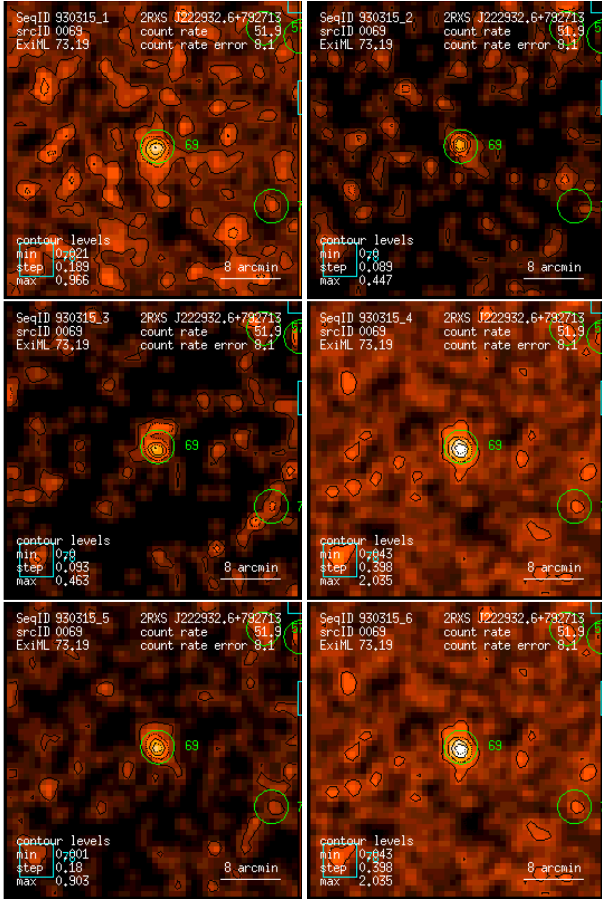
Figure 69: RASS 930315: detection 0069: band rate images, Gaussian filter: (1) PSPC channels 11 – 41, (2) 52 – 90, (3) 91 – 201, (4) 11 – 235, (5) 52 – 201, (6) 11 – 201. Broad band rates in counts/ks. Band rate contour levels in counts/ks/arcmin 2 .
