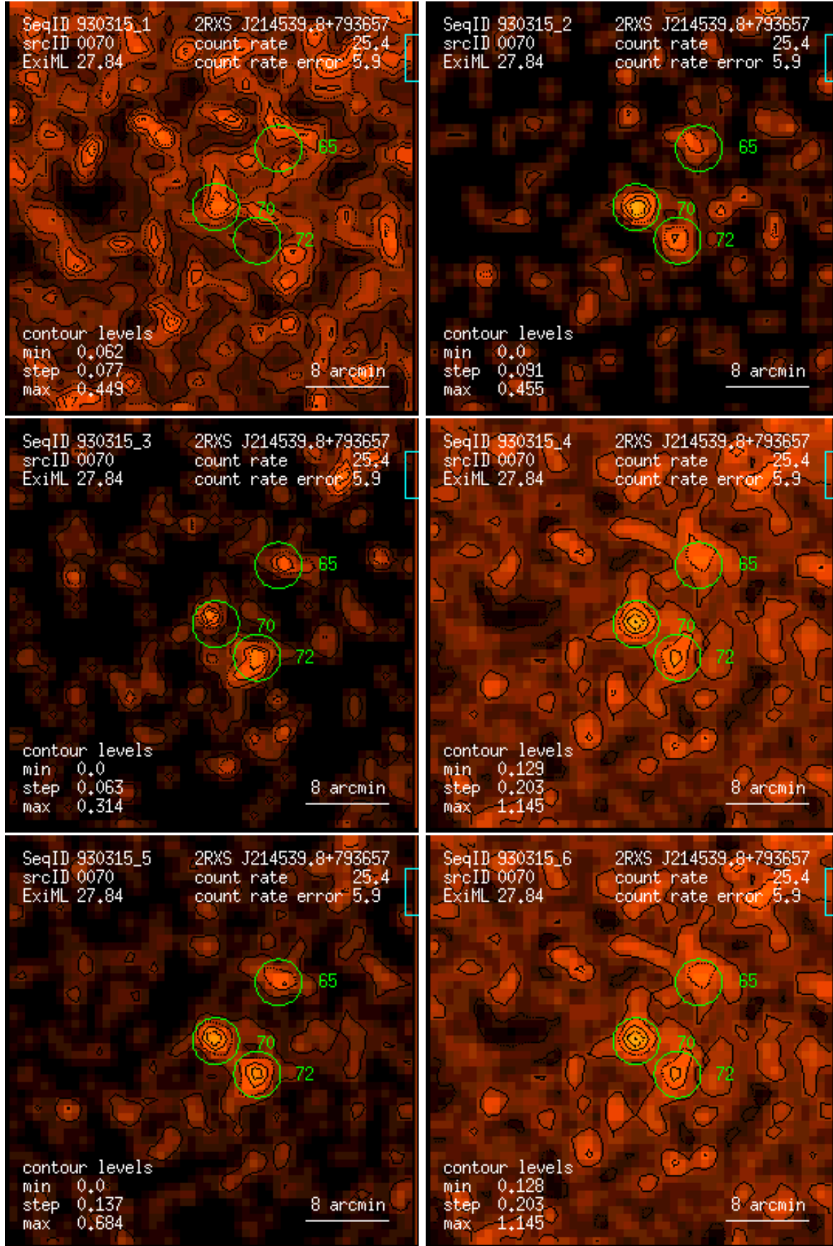
Figure 70: RASS 930315: detection 0070: band rate images, Gaussian filter: (1) PSPC channels 11 – 41, (2) 52 – 90, (3) 91 – 201, (4) 11 – 235, (5) 52 – 201, (6) 11 – 201. Broad band rates in counts/ks. Band rate contour levels in counts/ks/arcmin 2 .
