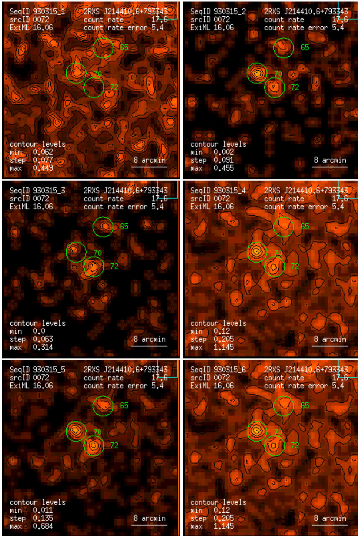
Figure 72: RASS 930315: detection 0072: band rate images, Gaussian filter: (1) PSPC channels 11 – 41, (2) 52 – 90, (3) 91 – 201, (4) 11 – 235, (5) 52 – 201, (6) 11 – 201. Broad band rates in counts/ks. Band rate contour levels in counts/ks/arcmin 2 .
