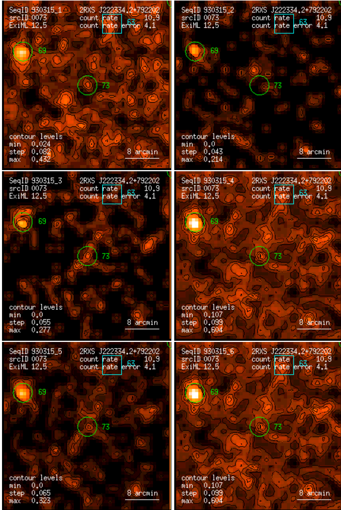
Figure 73: RASS 930315: detection 0073: band rate images, Gaussian filter: (1) PSPC channels 11 – 41, (2) 52 – 90, (3) 91 – 201, (4) 11 – 235, (5) 52 – 201, (6) 11 – 201. Broad band rates in counts/ks. Band rate contour levels in counts/ks/arcmin 2 .
