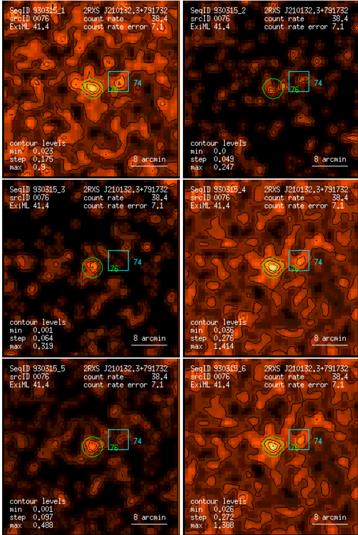
Figure 76: RASS 930315: detection 0076: band rate images, Gaussian filter: (1) PSPC channels 11 – 41, (2) 52 – 90, (3) 91 – 201, (4) 11 – 235, (5) 52 – 201, (6) 11 – 201. Broad band rates in counts/ks. Band rate contour levels in counts/ks/arcmin 2 .
